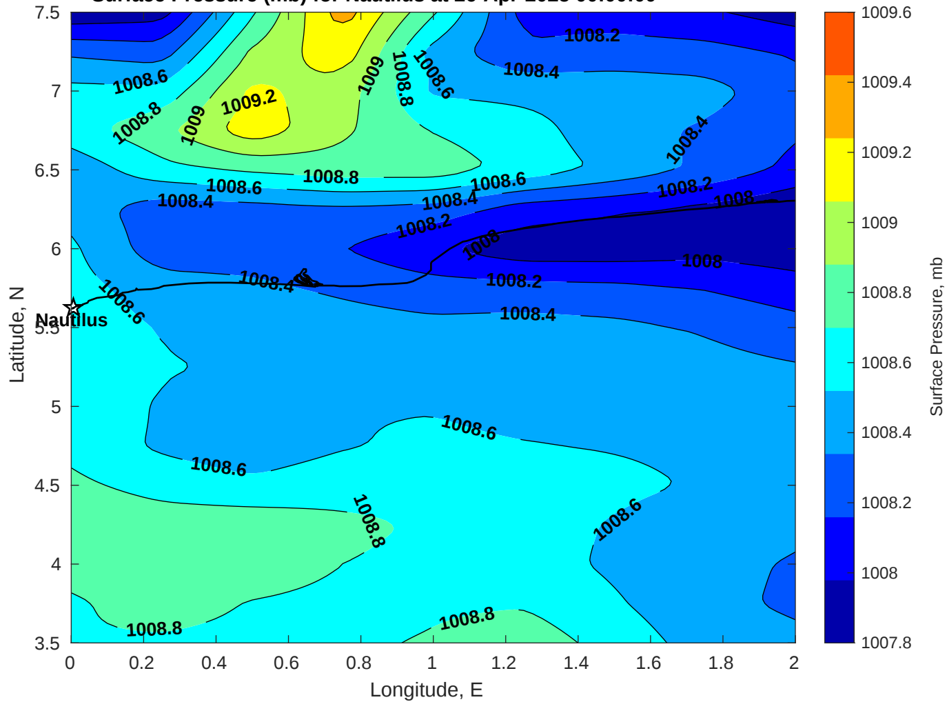
Surface Pressure (mb) for Nautilus at 26-Apr-2025 00:00:00
