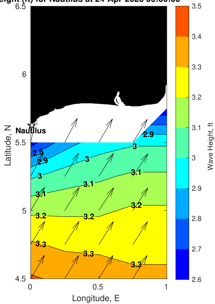
Wave Height (ft) for Nautilus at 24-Apr-2025 09:00:00
