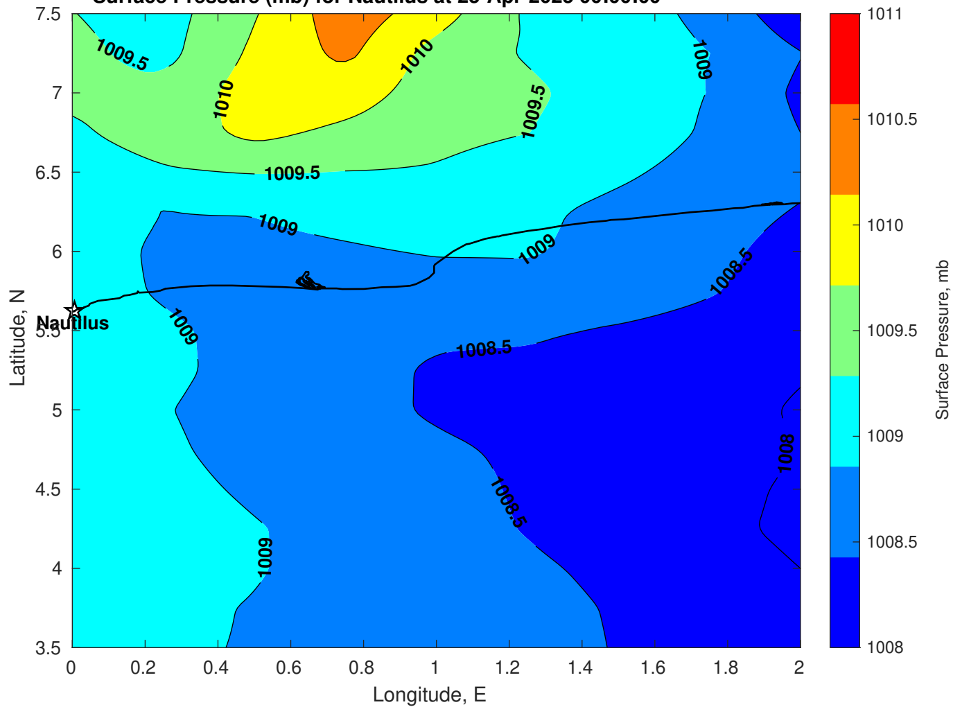
Surface Pressure (mb) for Nautilus at 25-Apr-2025 00:00:00
