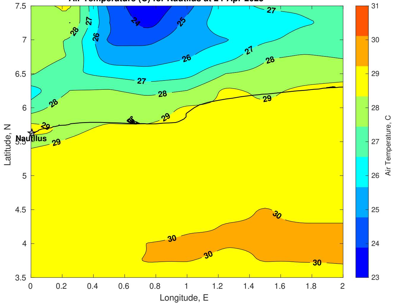
Air Temperature (C) for Nautilus at 24-Apr-2025
