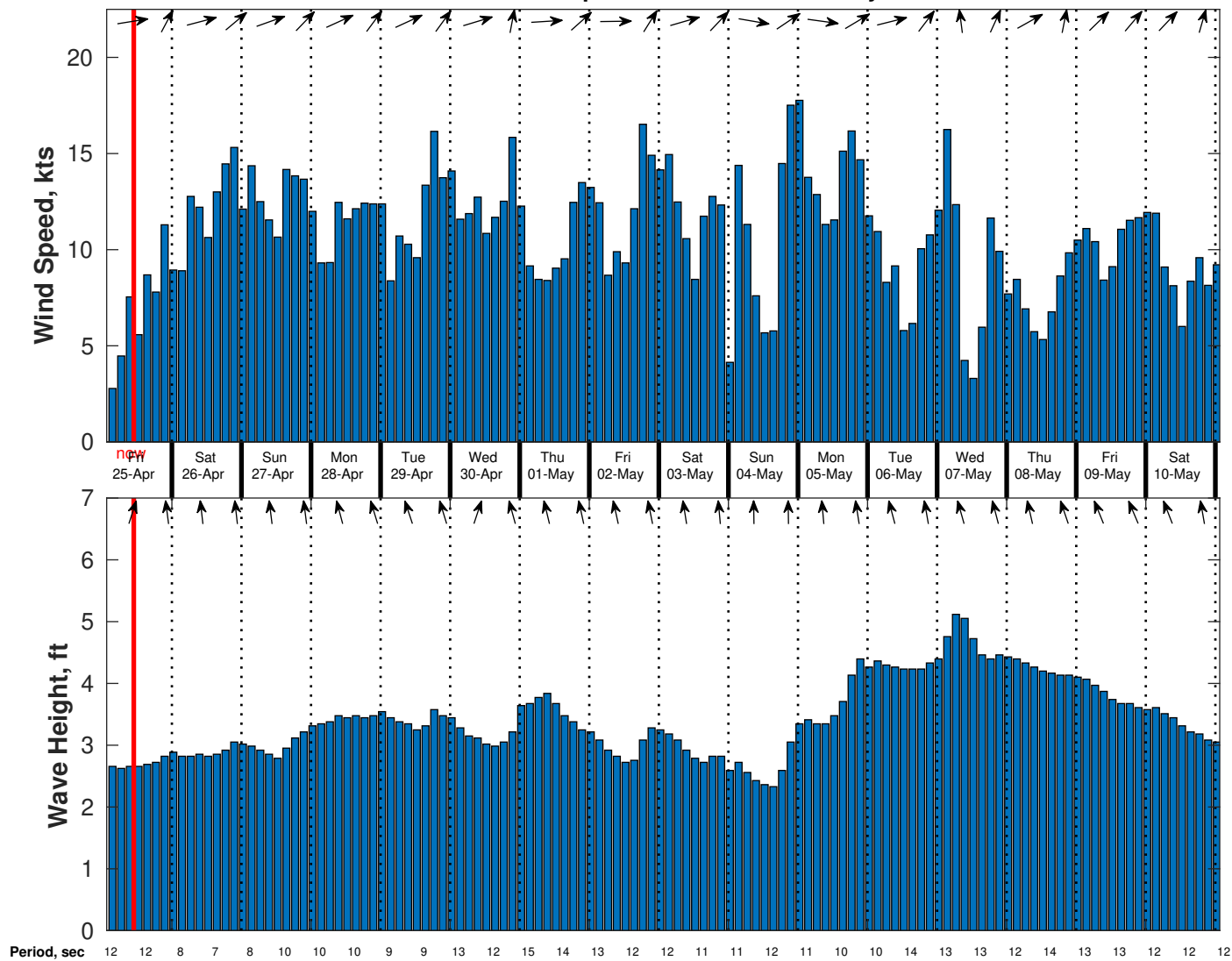
Wind & Wave Forecast for Nautilus from 24-Apr-2025 02:00:00 to 10-May-2025 02:00:00
