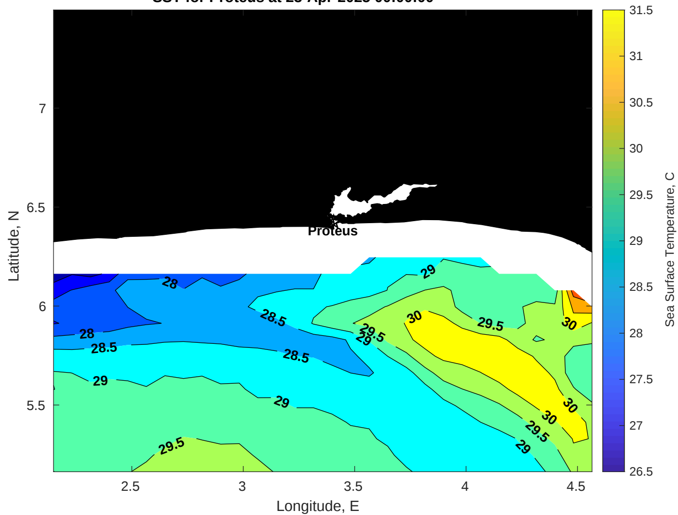
SST for Proteus at 23-Apr-2025 00:00:00
