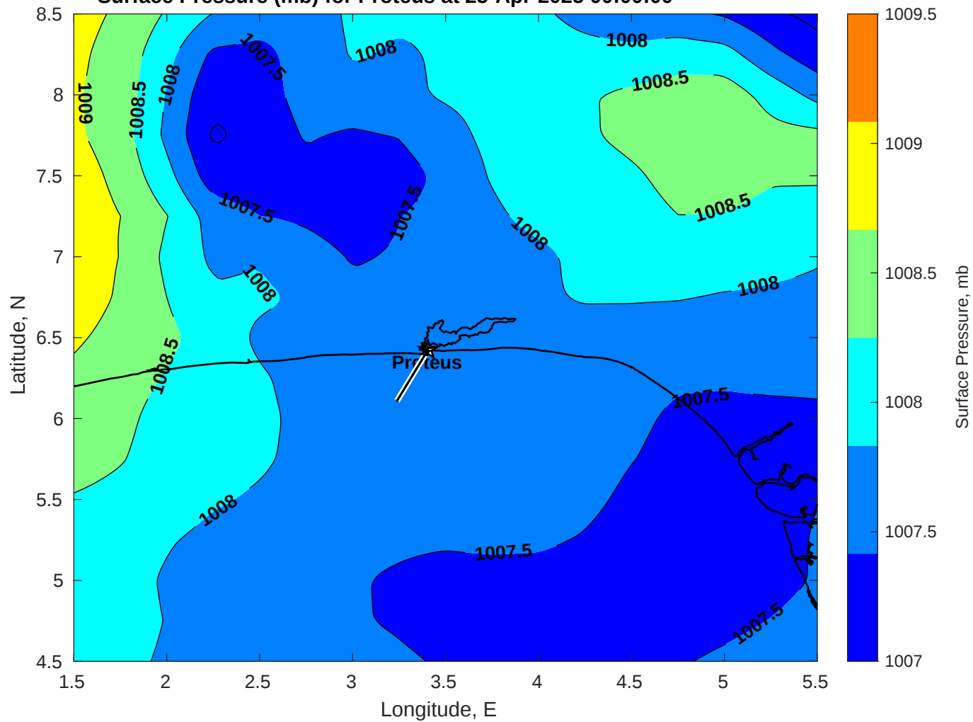
Surface Pressure (mb) for Proteus at 25-Apr-2025 00:00:00
