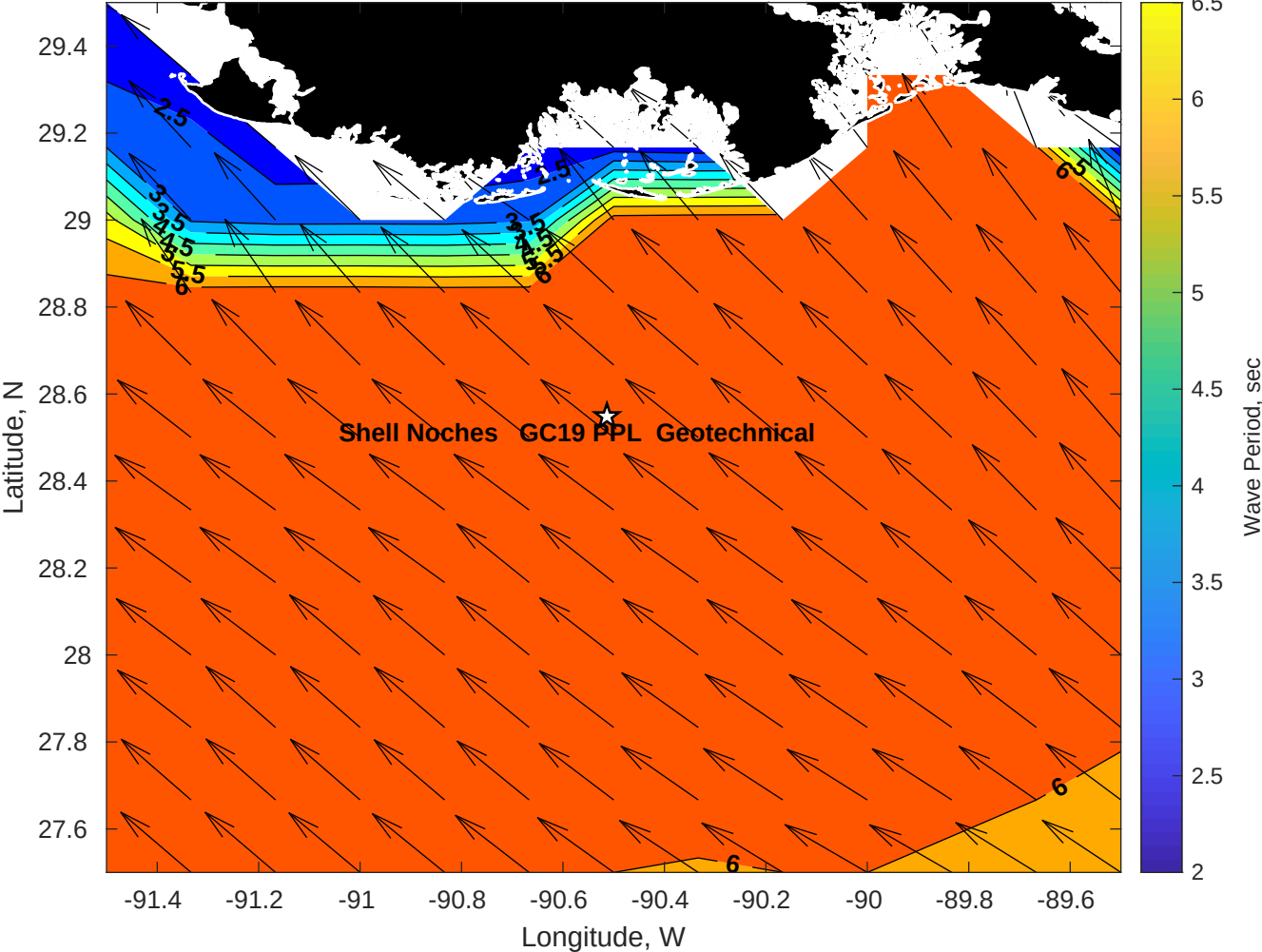
Wave Period (sec) for Shell Noches GC19 PPL Geotechnical at 24-Apr-2025 09:00:00
