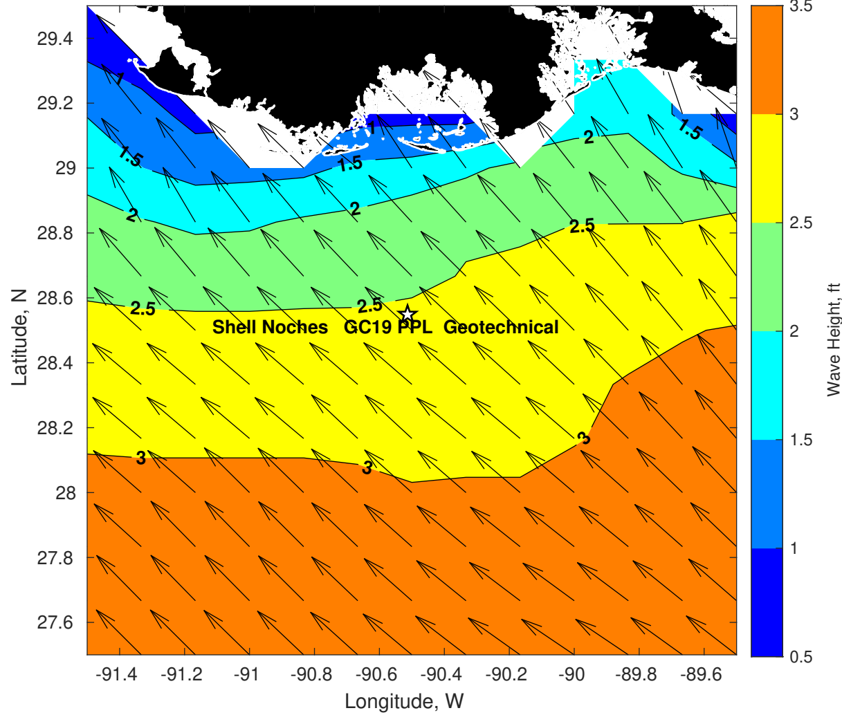
Wave Height (ft) for Shell Noches GC19 PPL Geotechnical at 24-Apr-2025 09:00:00
