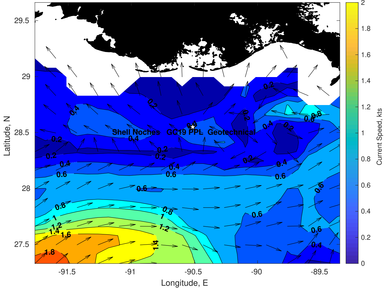
Surface Currents for Shell Noches GC19 PPL Geotechnical at 23-Apr-2025 00:00:00
