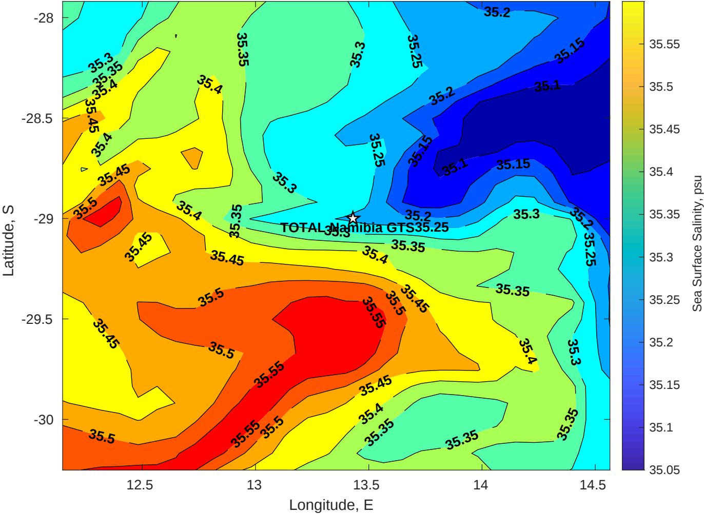
Surface Salinity for TOTAL Namibia GTS at 23-Apr-2025 00:00:00
