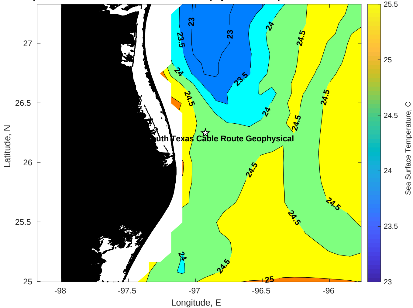
SST for Tampnet P2378 South Texas Cable Route Geophysical at 23-Apr-2025 00:00:00
