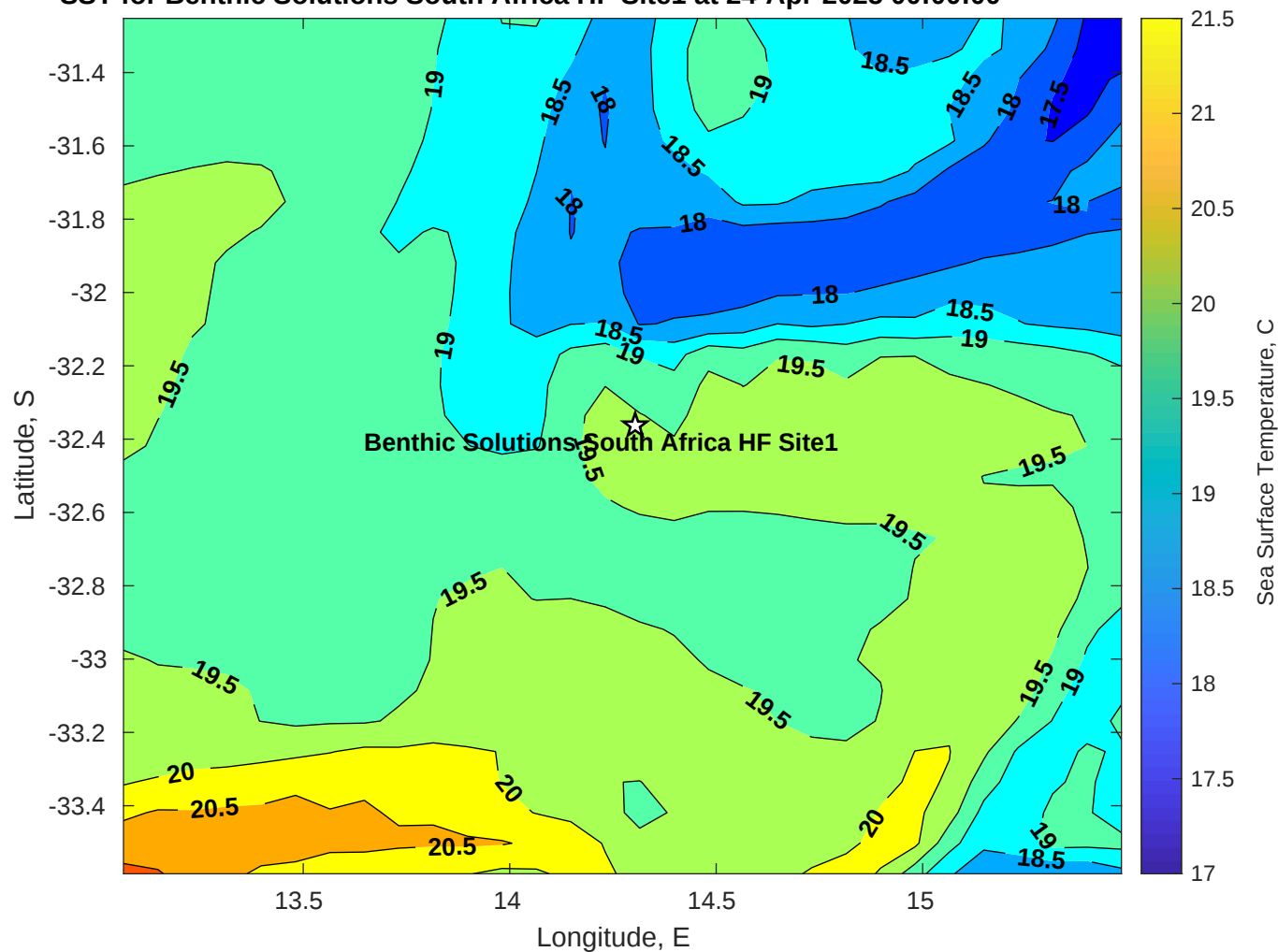
SST for Benthic Solutions South Africa HF Site1 at 24-Apr-2025 00:00:00
