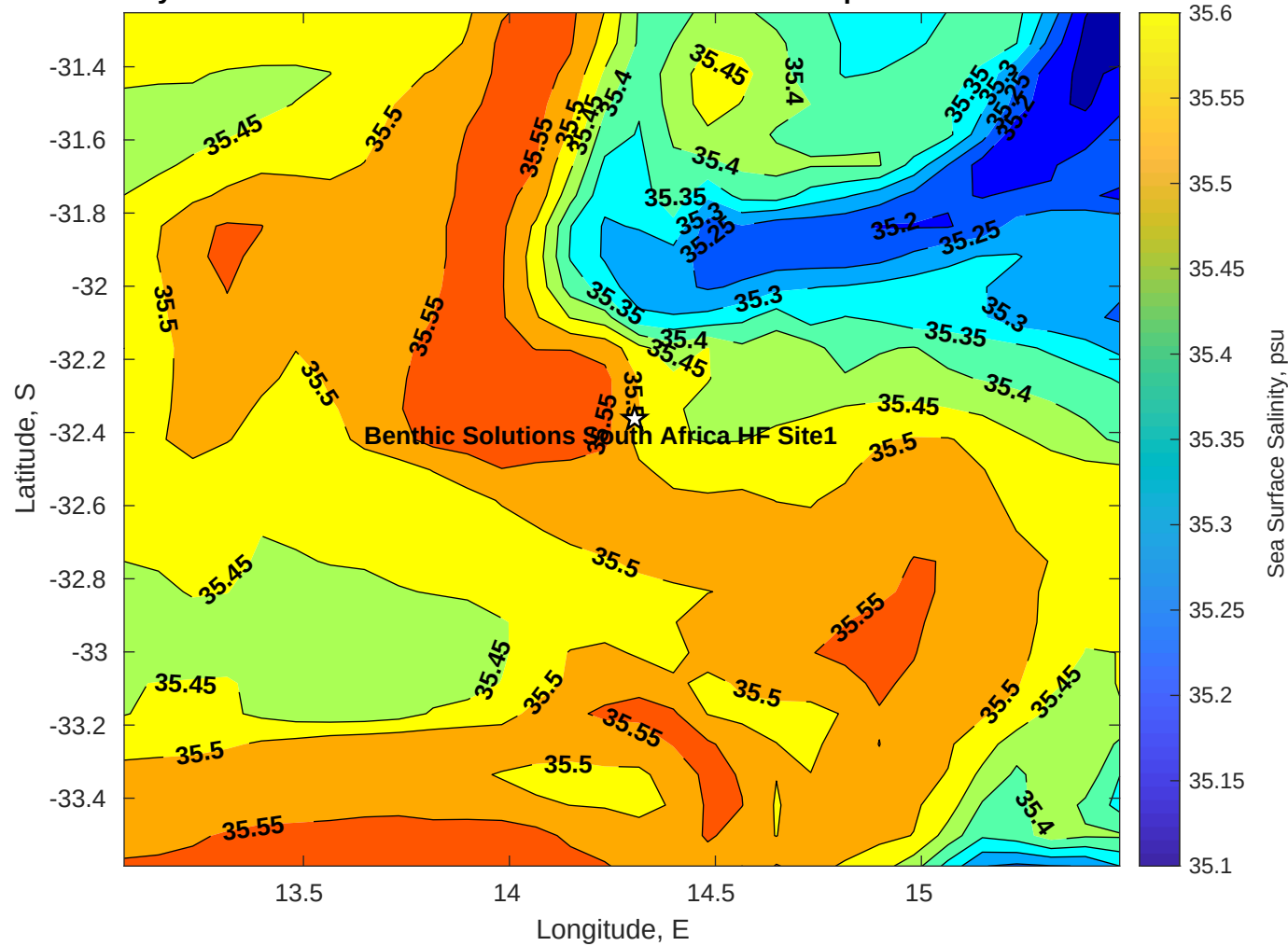
Surface Salinity for Benthic Solutions South Africa HF Site1 at 24-Apr-2025 00:00:00
