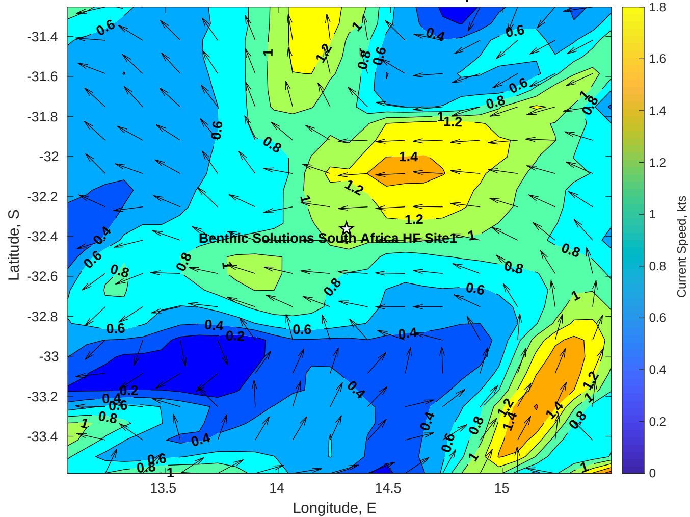
Surface Currents for Benthic Solutions South Africa HF Site1 at 24-Apr-2025 00:00:00
