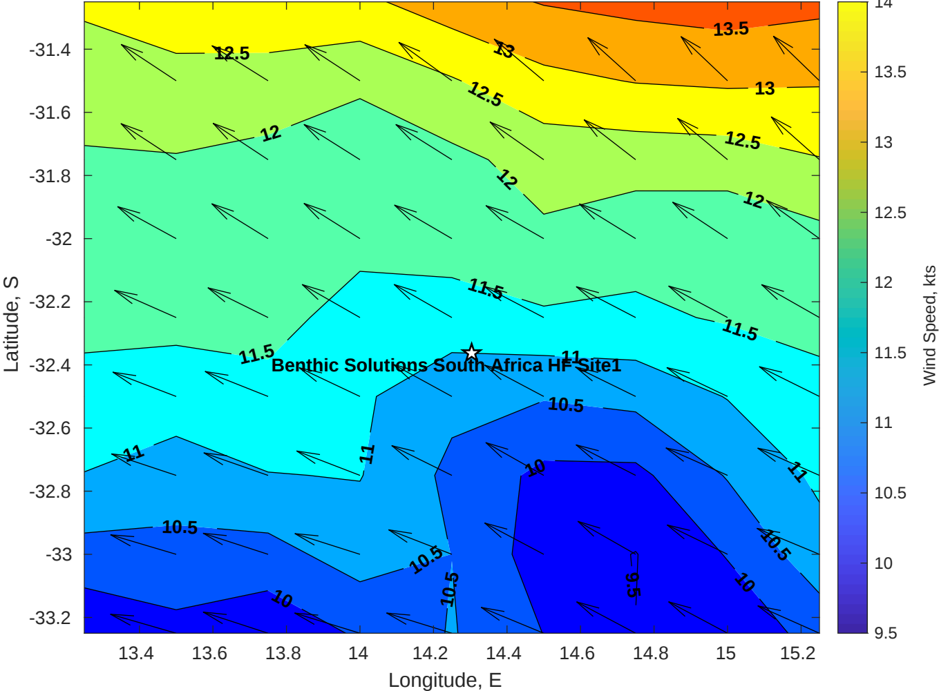
Winds (kts) for Benthic Solutions South Africa HF Site1 at 25-Apr-2025 09:00:00
