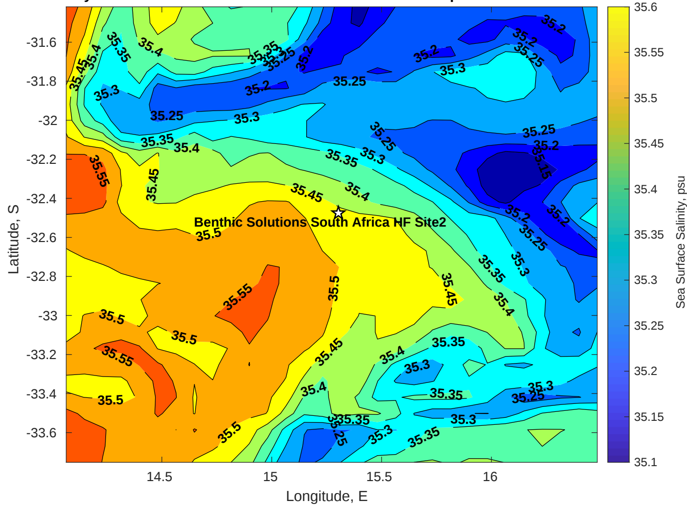
Surface Salinity for Benthic Solutions South Africa HF Site2 at 24-Apr-2025 00:00:00
