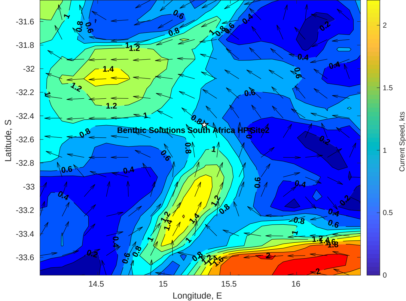
Surface Currents for Benthic Solutions South Africa HF Site2 at 24-Apr-2025 00:00:00
