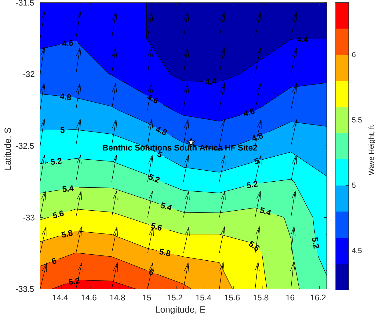
Wave Height (ft) for Benthic Solutions South Africa HF Site2 at 25-Apr-2025 09:00:00
