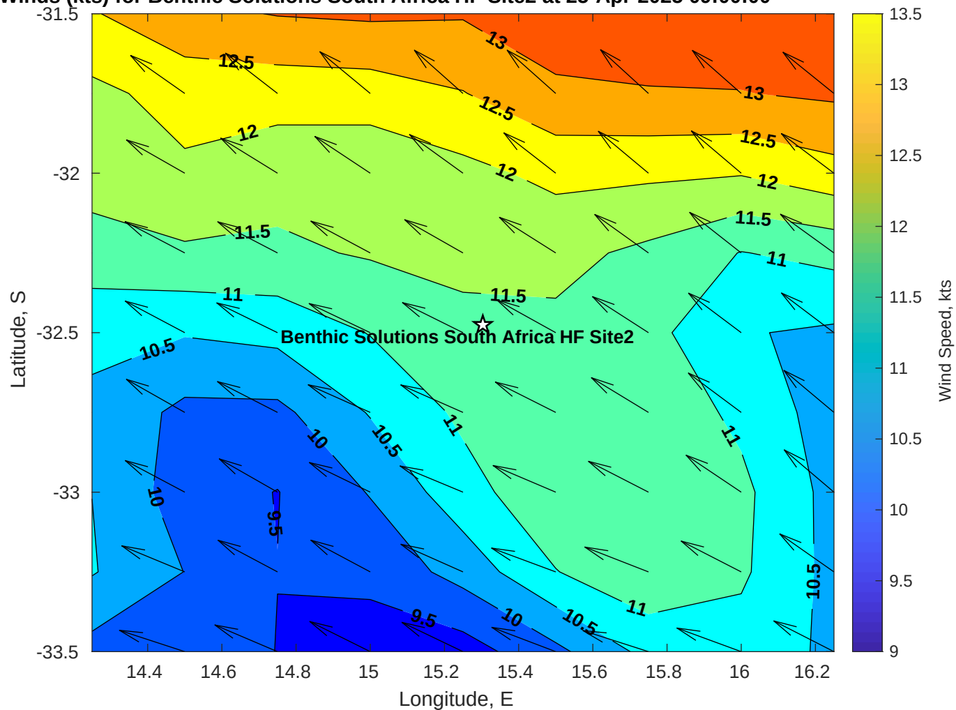
Winds (kts) for Benthic Solutions South Africa HF Site2 at 25-Apr-2025 09:00:00
