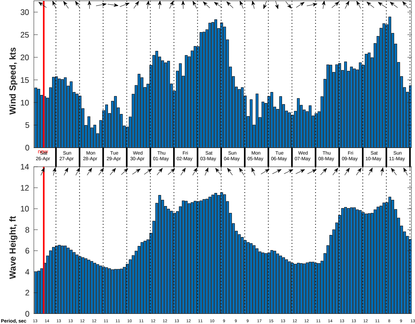
Wind & Wave Forecast for Benthic Solutions South Africa HF Site2 from 25-Apr-2025 02:00:00 to 11-May-2025 02:00:00
