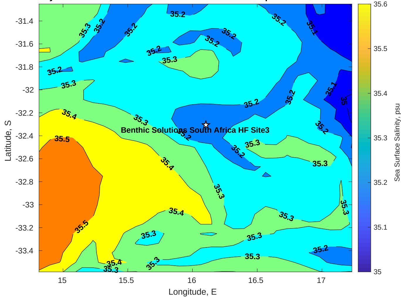
Surface Salinity for Benthic Solutions South Africa HF Site3 at 24-Apr-2025 00:00:00
