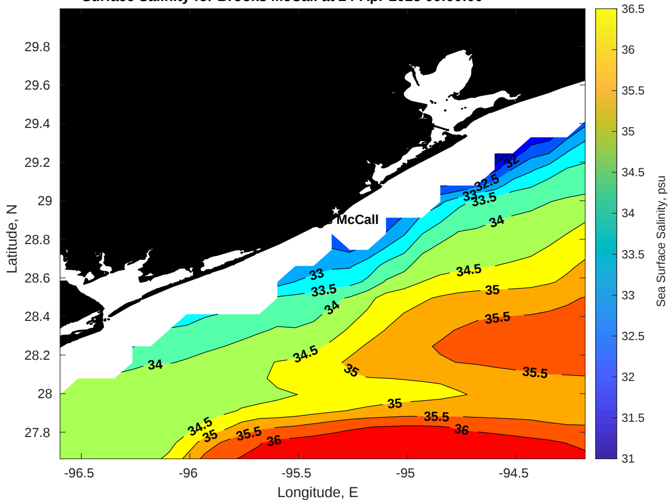
Surface Salinity for Brooks McCall at 24-Apr-2025 00:00:00
