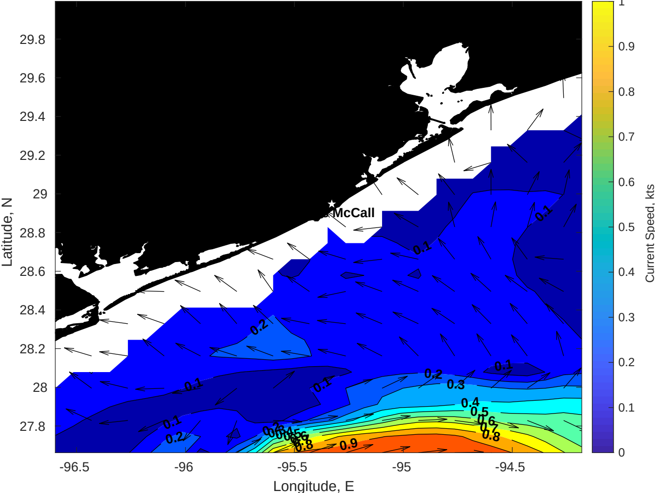
Surface Currents for Brooks McCall at 24-Apr-2025 00:00:00
