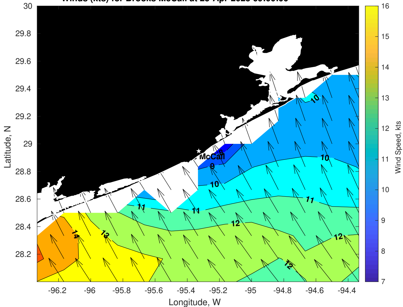
Winds (kts) for Brooks McCall at 25-Apr-2025 09:00:00
