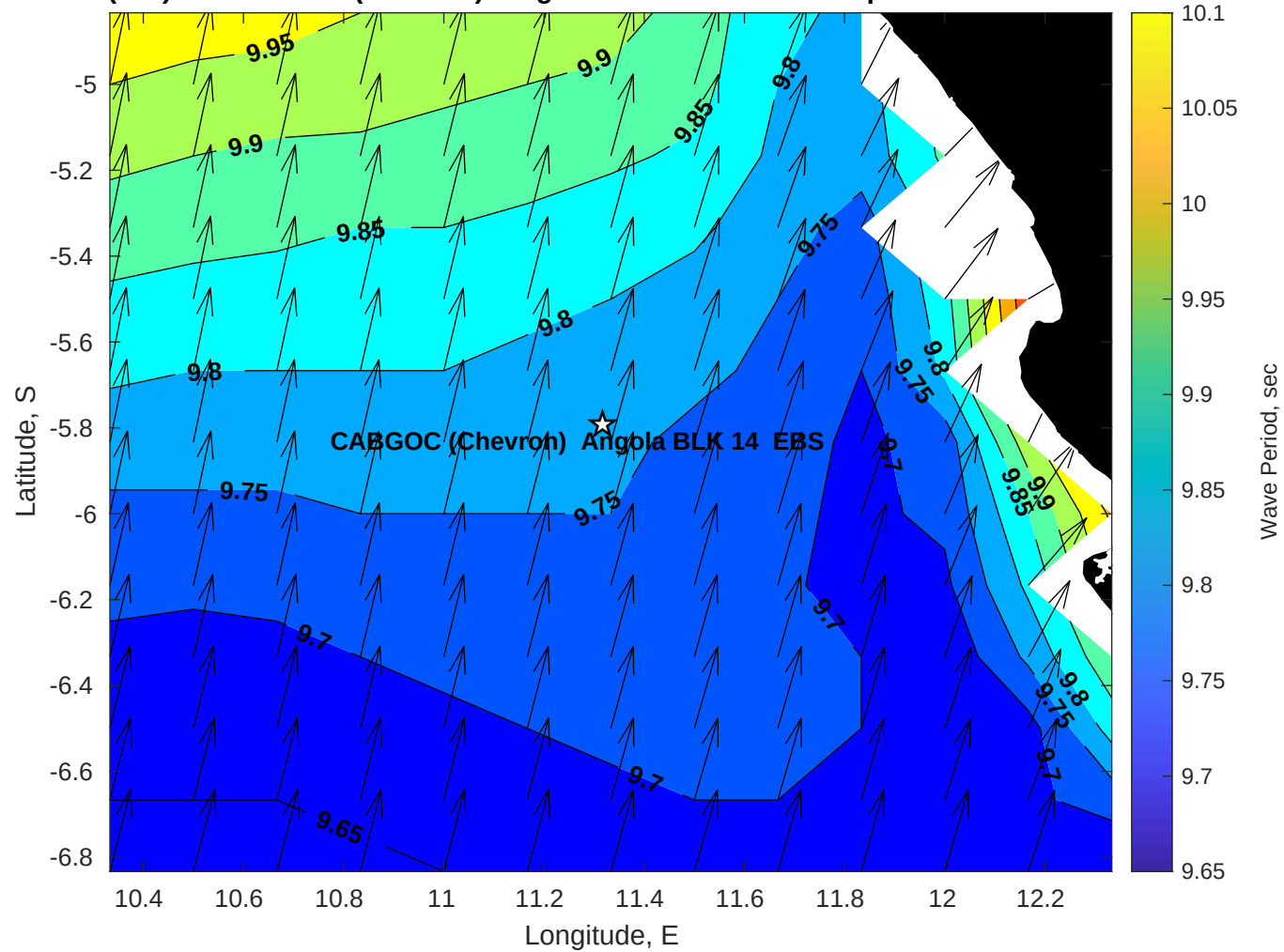
Wave Period (sec) for CABGOC (Chevron) Angola BLK 14 EBS at 25-Apr-2025 09:00:00
