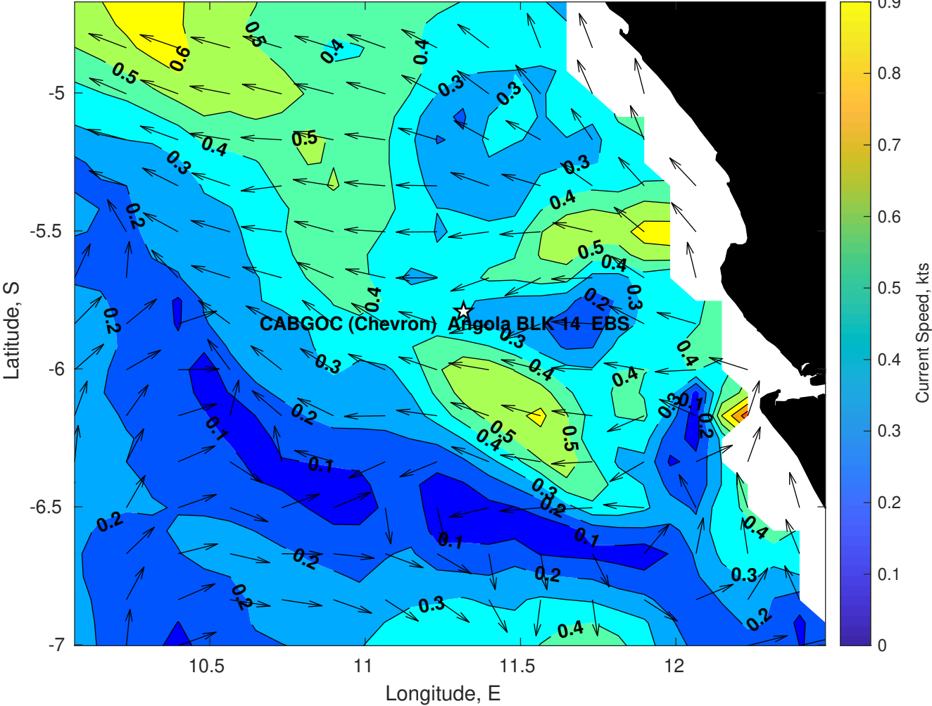
Surface Currents for CABGOC (Chevron) Angola BLK 14 EBS at 24-Apr-2025 00:00:00
