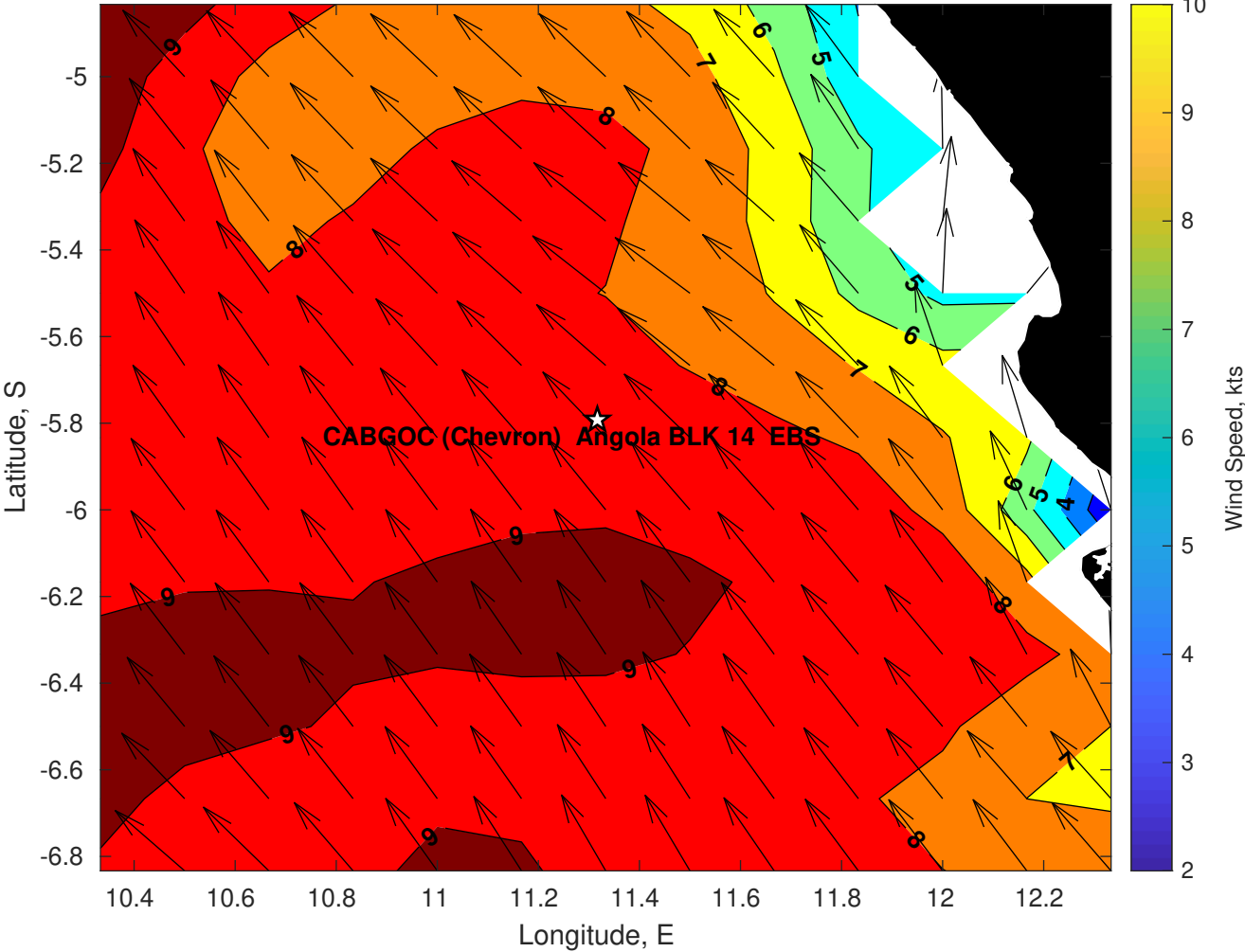
Winds (kts) for CABGOC (Chevron) Angola BLK 14 EBS at 25-Apr-2025 09:00:00
