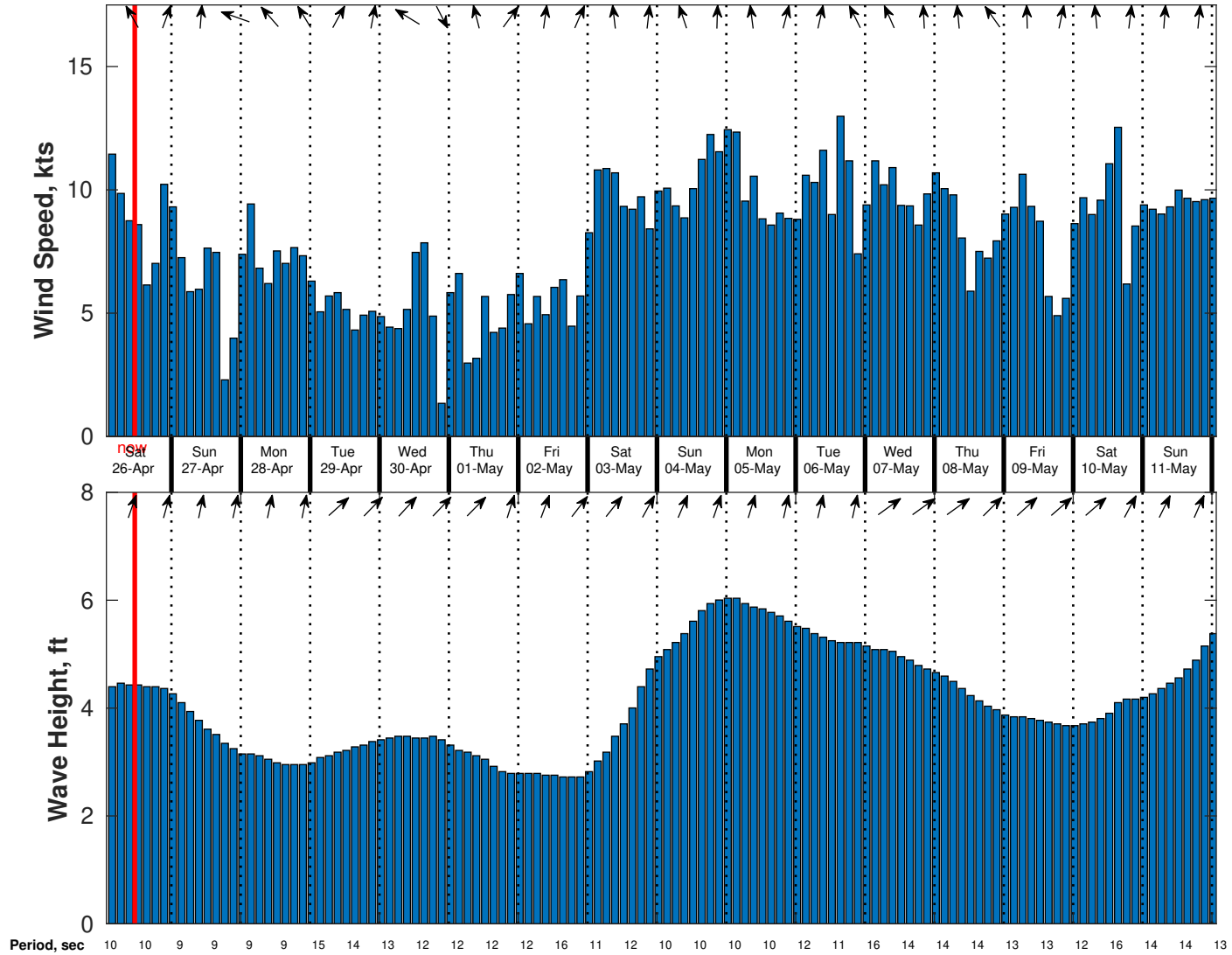
Wind & Wave Forecast for CABGOC (Chevron) Angola BLK 14 EBS from 25-Apr-2025 02:00:00 to 11-May-2025 02:00:00
