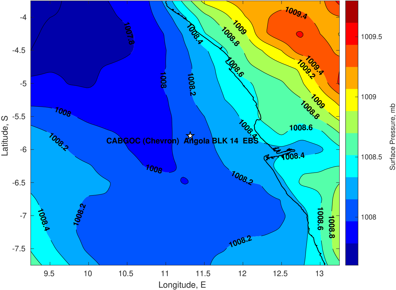
Surface Pressure (mb) for CABGOC (Chevron) Angola BLK 14 EBS at 27-Apr-2025 00:00:00
