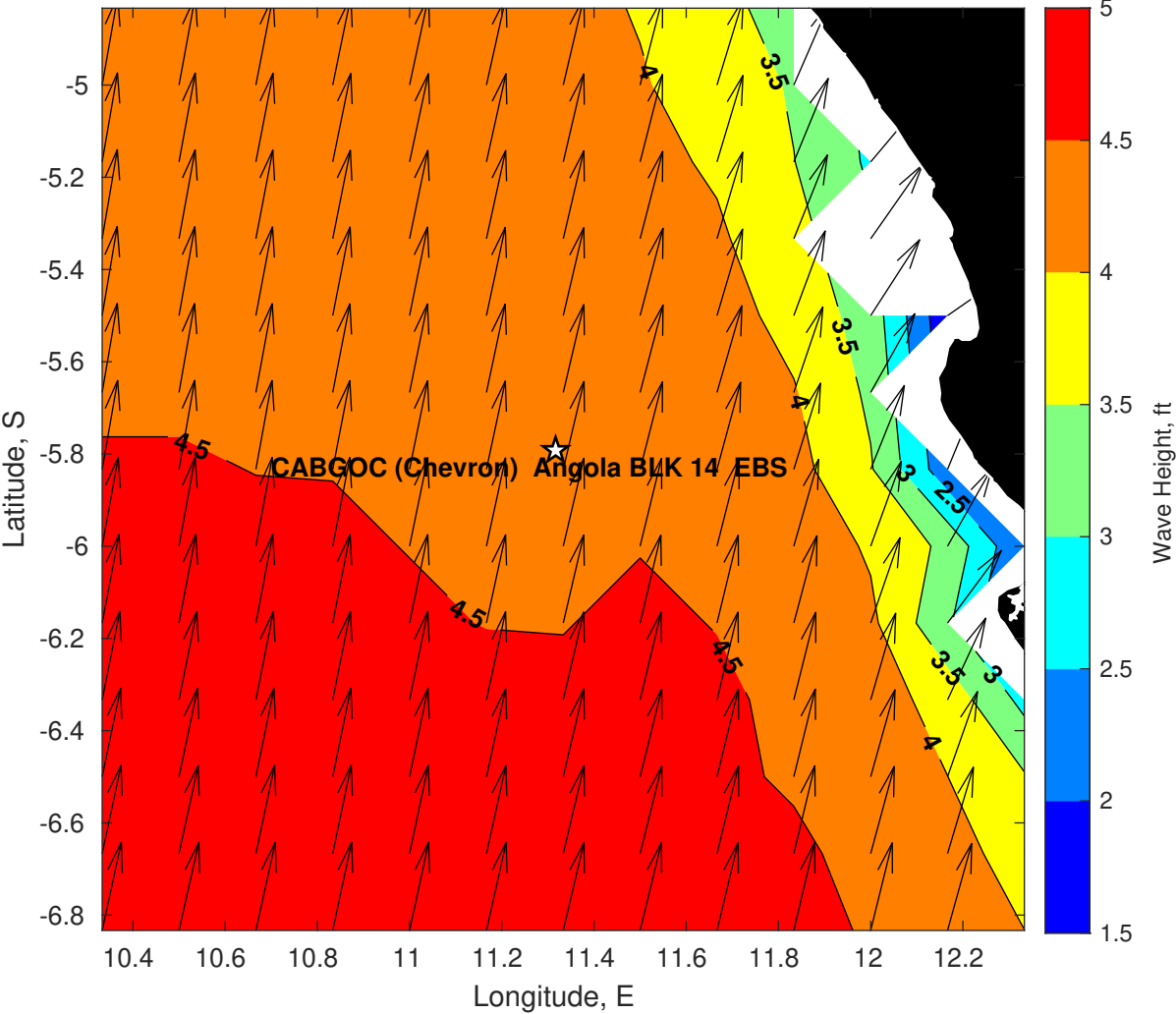
Wave Height (ft) for CABGOC (Chevron) Angola BLK 14 EBS at 25-Apr-2025 09:00:00
