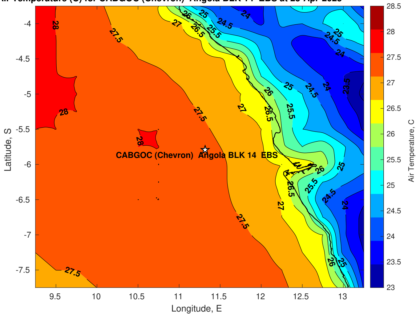
Air Temperature (C) for CABGOC (Chevron) Angola BLK 14 EBS at 25-Apr-2025
