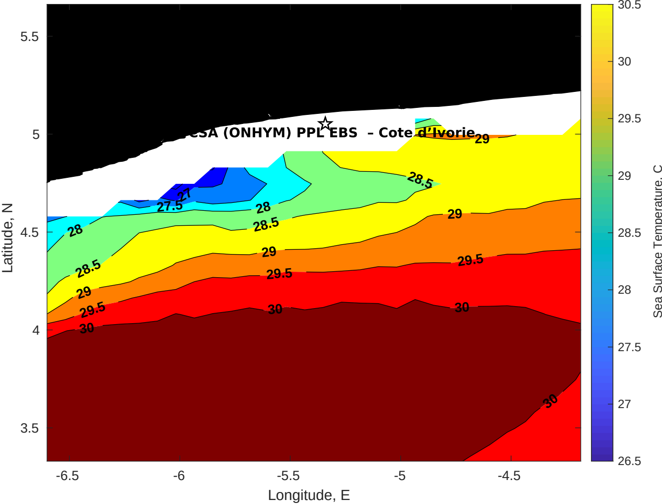
SST for CSA (ONHYM) PPL EBS - Cote d'Ivoire at 24-Apr-2025 00:00:00
