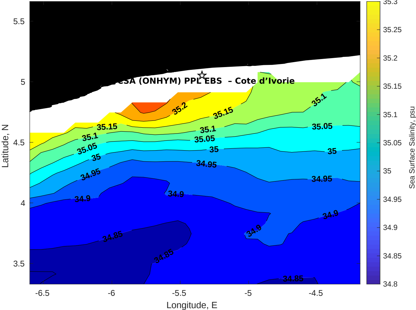
Surface Salinity for CSA (ONHYM) PPL EBS - Cote d'Ivoire at 24-Apr-2025 00:00:00
