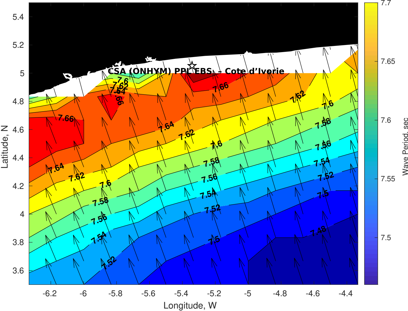
Wave Period (sec) for CSA (ONHYM) PPL EBS - Cote d'Ivoire at 25-Apr-2025 09:00:00
