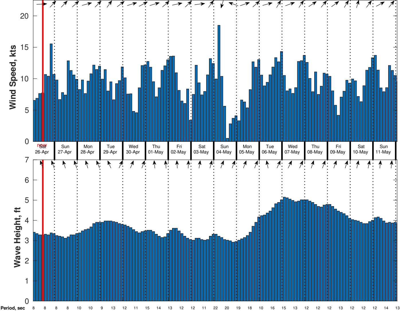
Wind & Wave Forecast for CSA (ONHYM) PPL EBS - Cote d'Ivoire from 25-Apr-2025 01:00:00 to 11-May-2025 01:00:00
