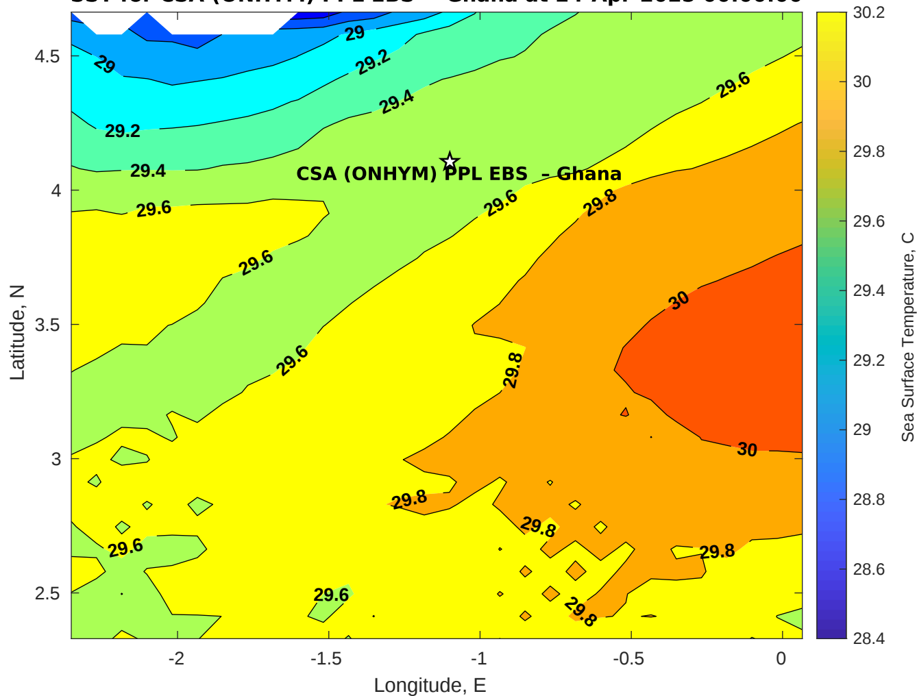
SST for CSA (ONHYM) PPL EBS - Ghana at 24-Apr-2025 00:00:00
