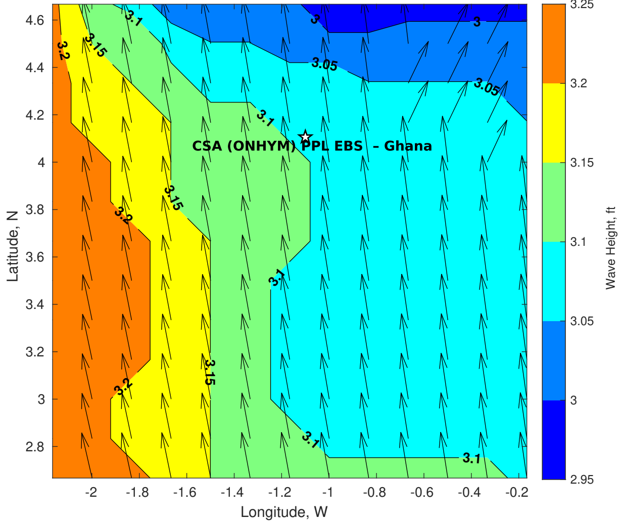
Wave Height (ft) for CSA (ONHYM) PPL EBS - Ghana at 25-Apr-2025 09:00:00
