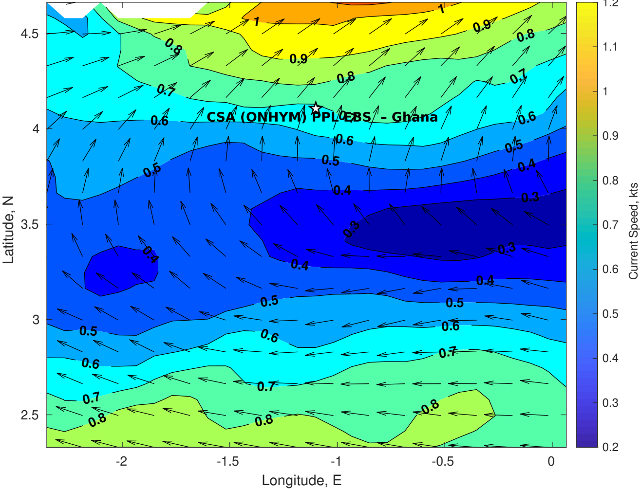
Surface Currents for CSA (ONHYM) PPL EBS - Ghana at 24-Apr-2025 00:00:00
