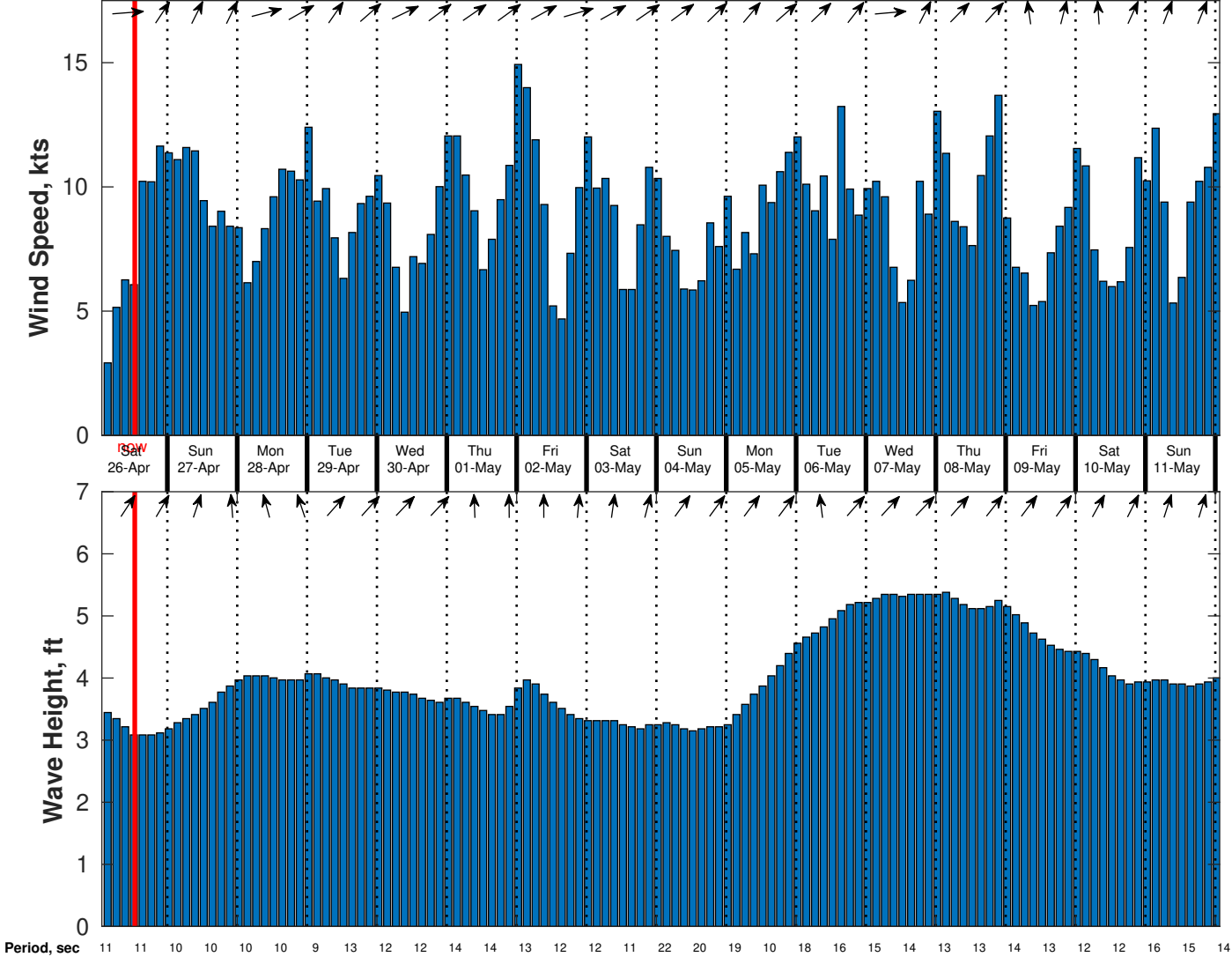
Wind & Wave Forecast for CSA (ONHYM) PPL EBS - Ghana from 25-Apr-2025 02:00:00 to 11-May-2025 02:00:00
