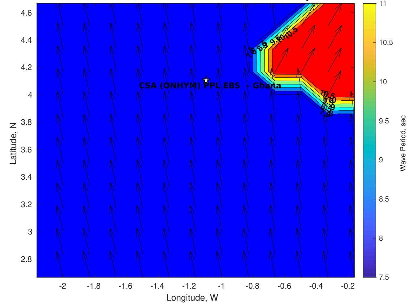
Wave Period (sec) for CSA (ONHYM) PPL EBS - Ghana at 25-Apr-2025 09:00:00
