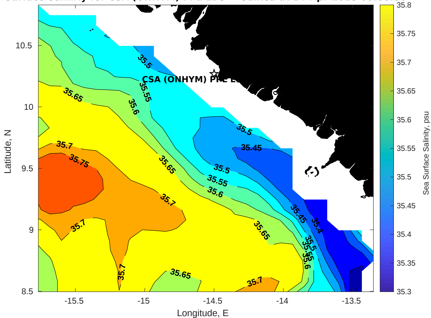
Surface Salinity for CSA (ONHYM) PPL EBS - Guinea at 24-Apr-2025 00:00:00
