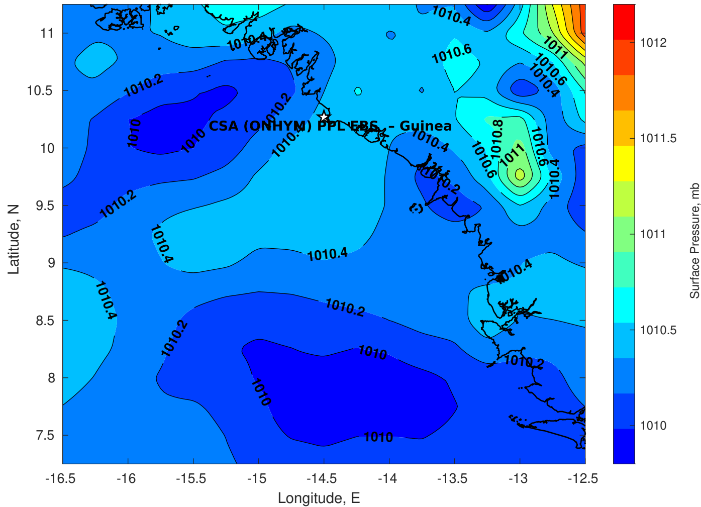
Surface Pressure (mb) for CSA (ONHYM) PPL EBS - Guinea at 25-Apr-2025 00:00:00
