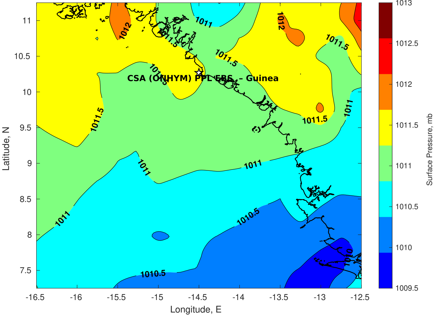
Surface Pressure (mb) for CSA (ONHYM) PPL EBS - Guinea at 27-Apr-2025 00:00:00
