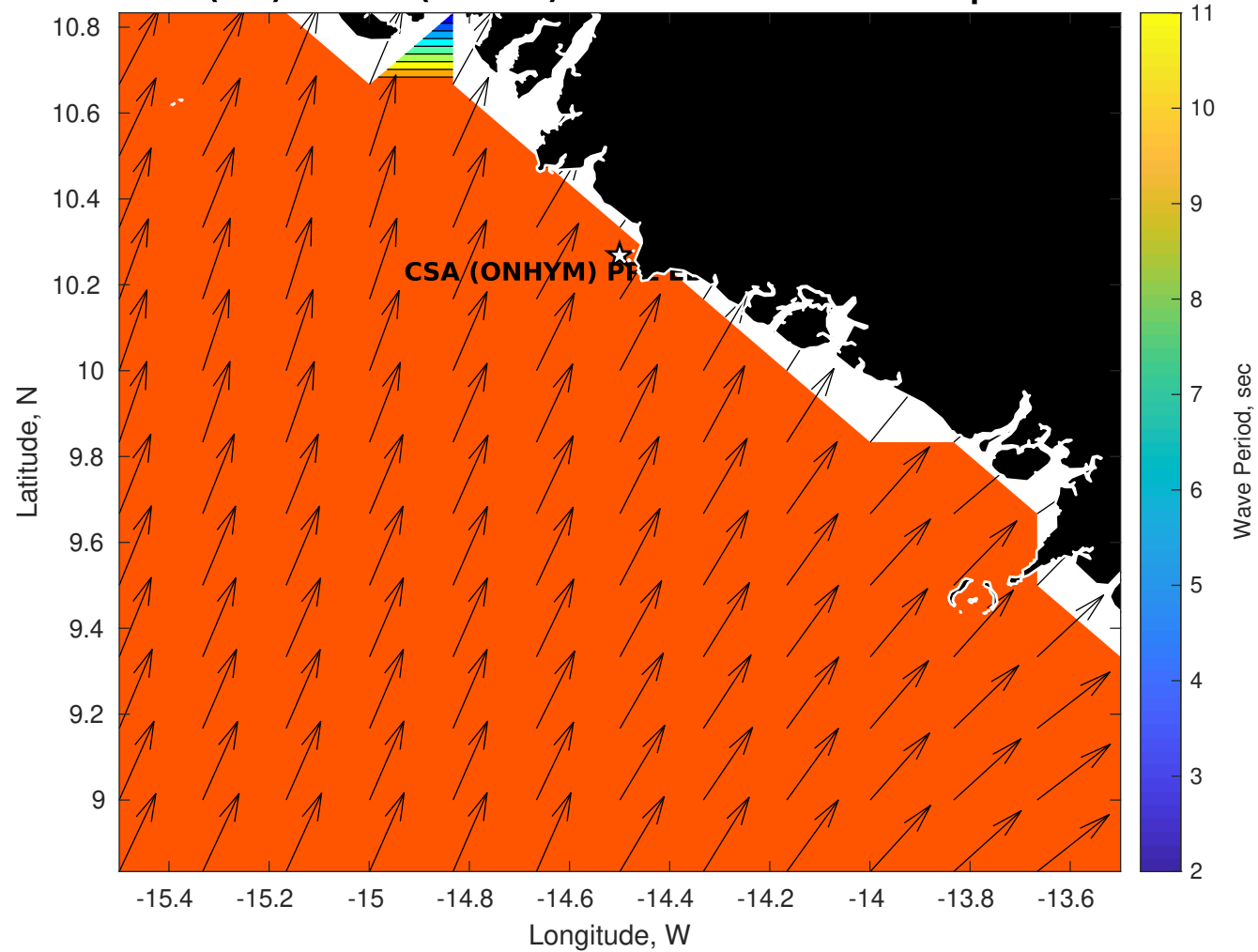
Wave Period (sec) for CSA (ONHYM) PPL EBS - Guinea at 25-Apr-2025 09:00:00
