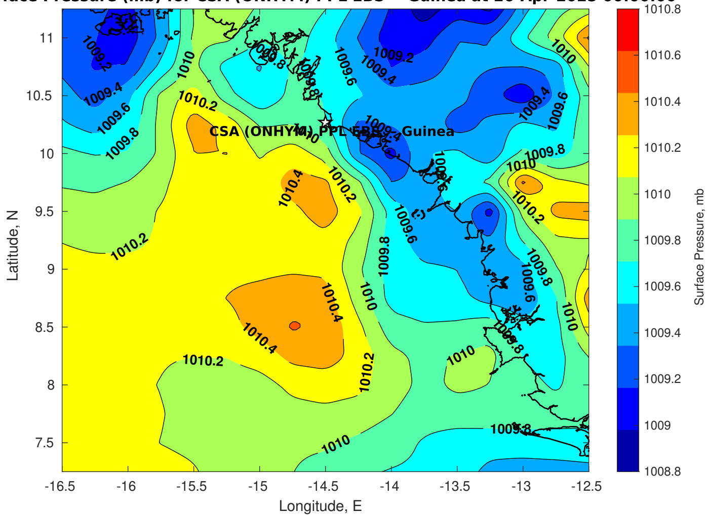
Surface Pressure (mb) for CSA (ONHYM) PPL EBS - Guinea at 26-Apr-2025 00:00:00
