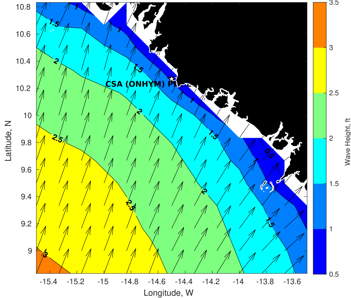
Wave Height (ft) for CSA (ONHYM) PPL EBS - Guinea at 25-Apr-2025 09:00:00
