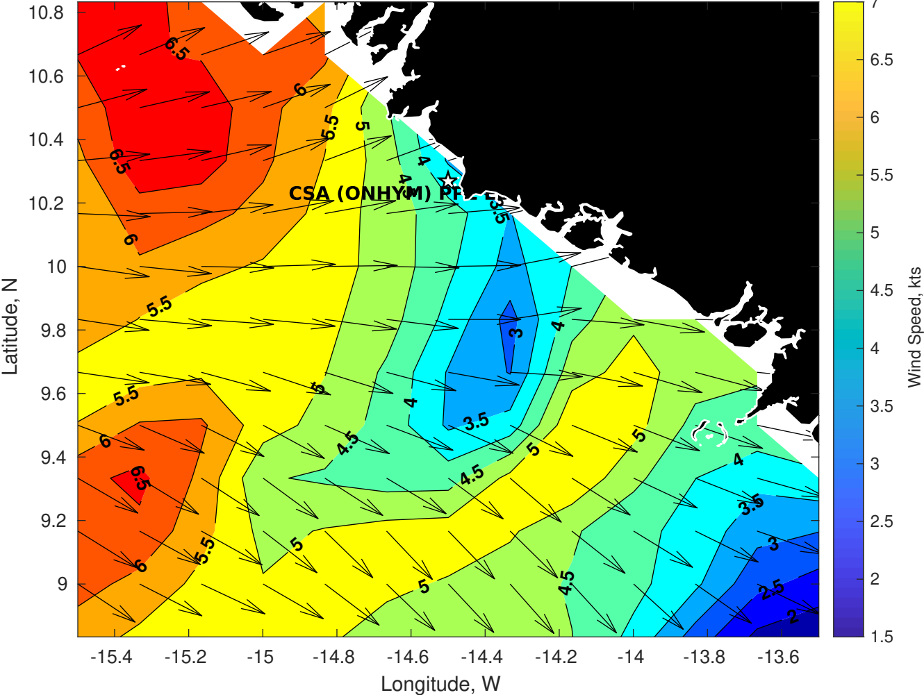
Winds (kts) for CSA (ONHYM) PPL EBS - Guinea at 25-Apr-2025 09:00:00
