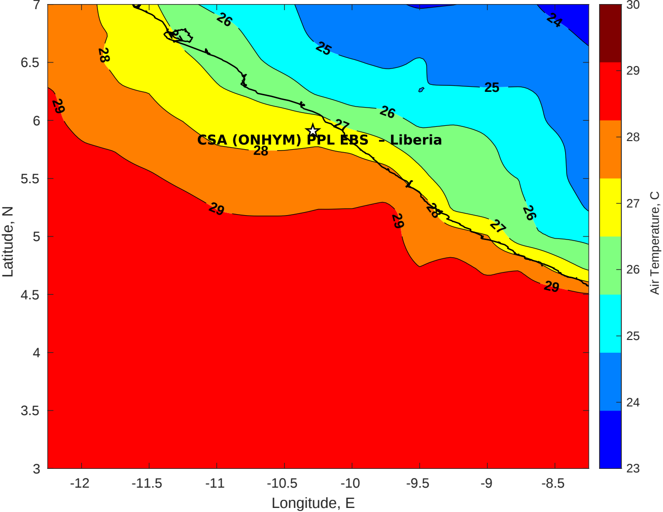
Air Temperature (C) for CSA (ONHYM) PPL EBS - Liberia at 25-Apr-2025
