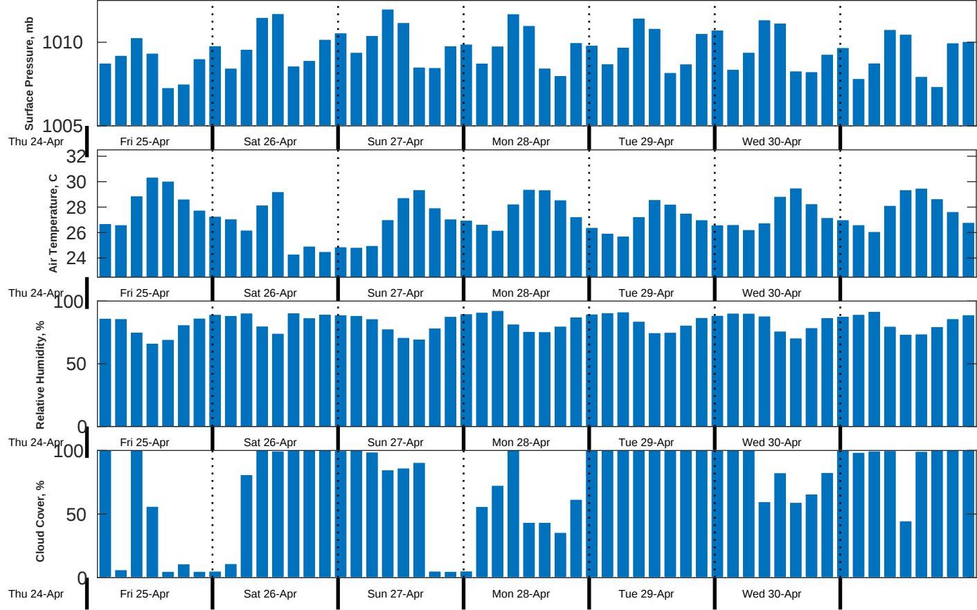
Met Forecast for CSA (ONHYM) PPL EBS - Liberia from 25-Apr-2025 00:00:00 to 02-May-2025 00:00:00
