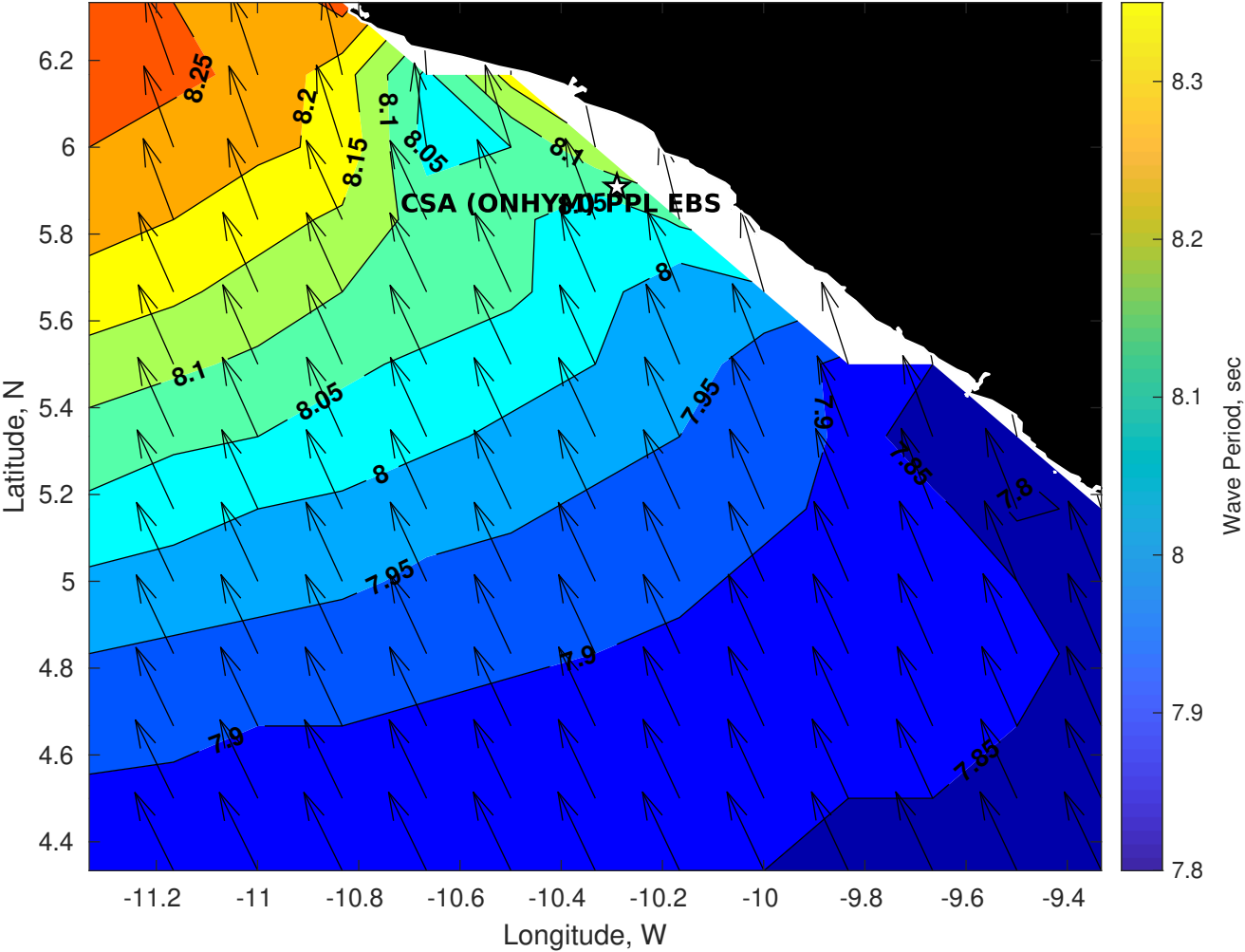
Wave Period (sec) for CSA (ONHYM) PPL EBS - Liberia at 25-Apr-2025 09:00:00
