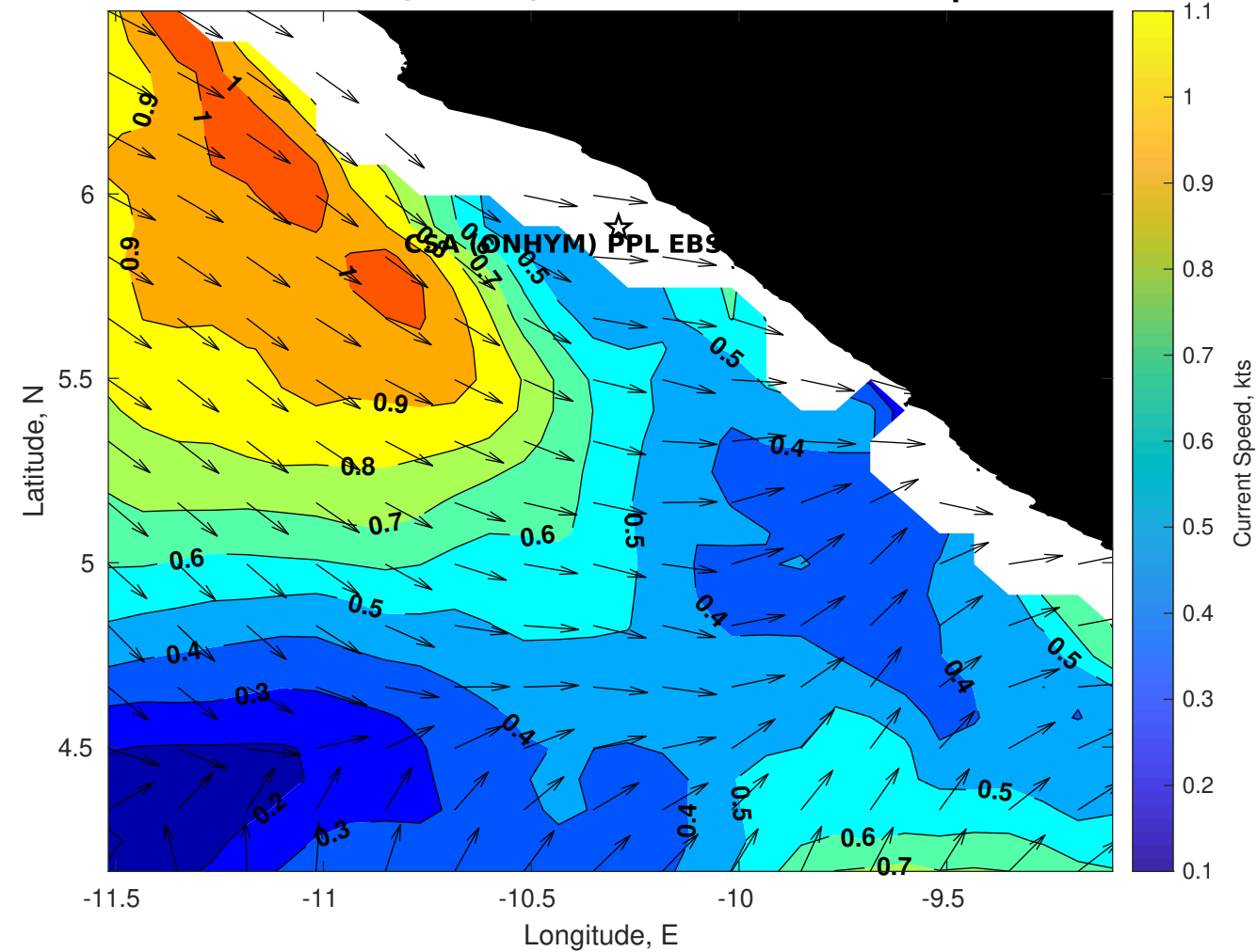
Surface Currents for CSA (ONHYM) PPL EBS - Liberia at 24-Apr-2025 00:00:00
