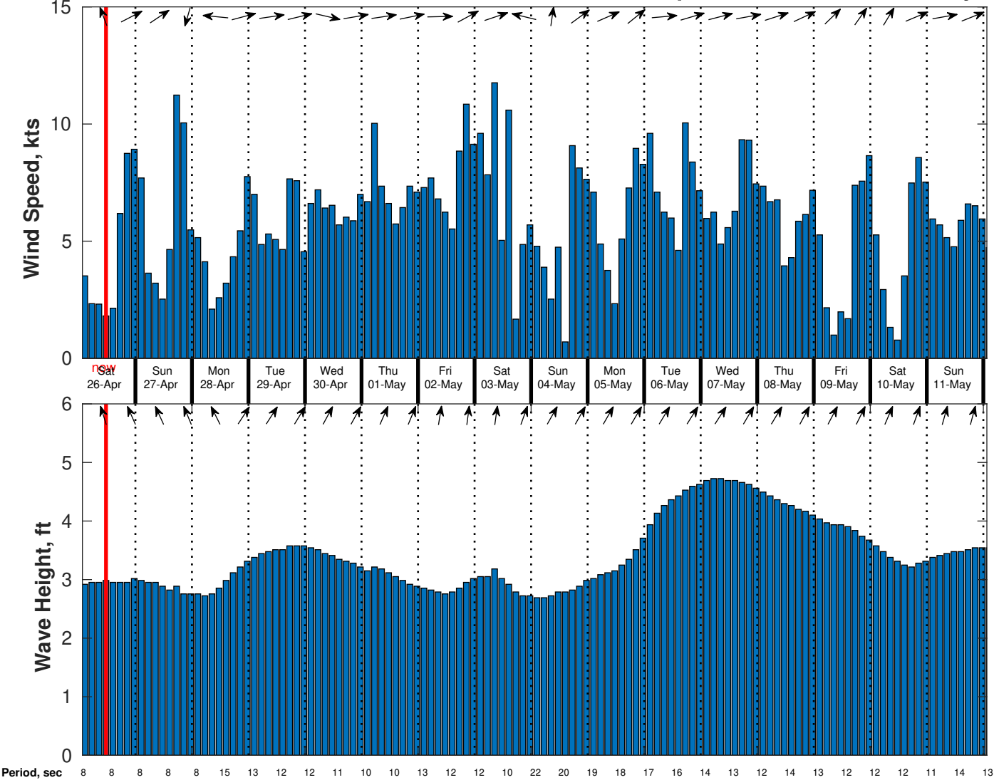
Wind & Wave Forecast for CSA (ONHYM) PPL EBS - Liberia from 25-Apr-2025 01:00:00 to 11-May-2025 01:00:00
