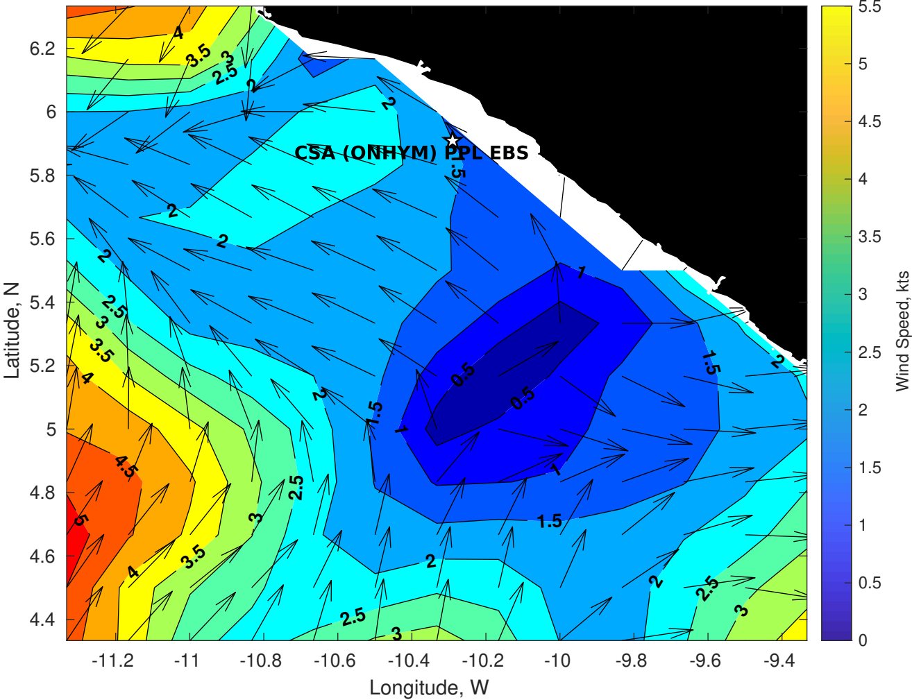
Winds (kts) for CSA (ONHYM) PPL EBS - Liberia at 25-Apr-2025 09:00:00
