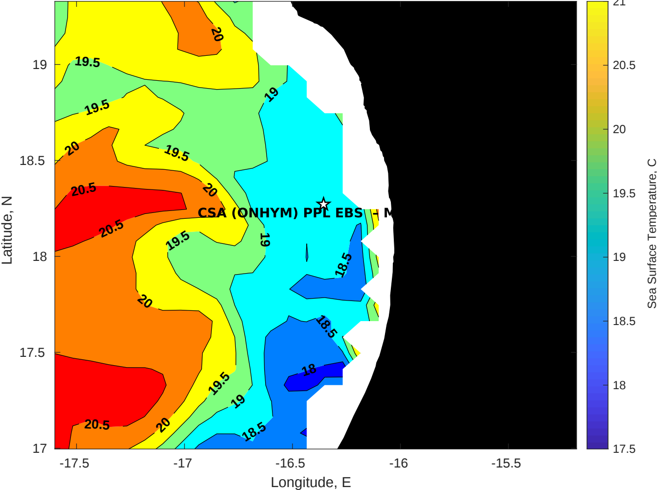
SST for CSA (ONHYM) PPL EBS - Mauritania at 24-Apr-2025 00:00:00
