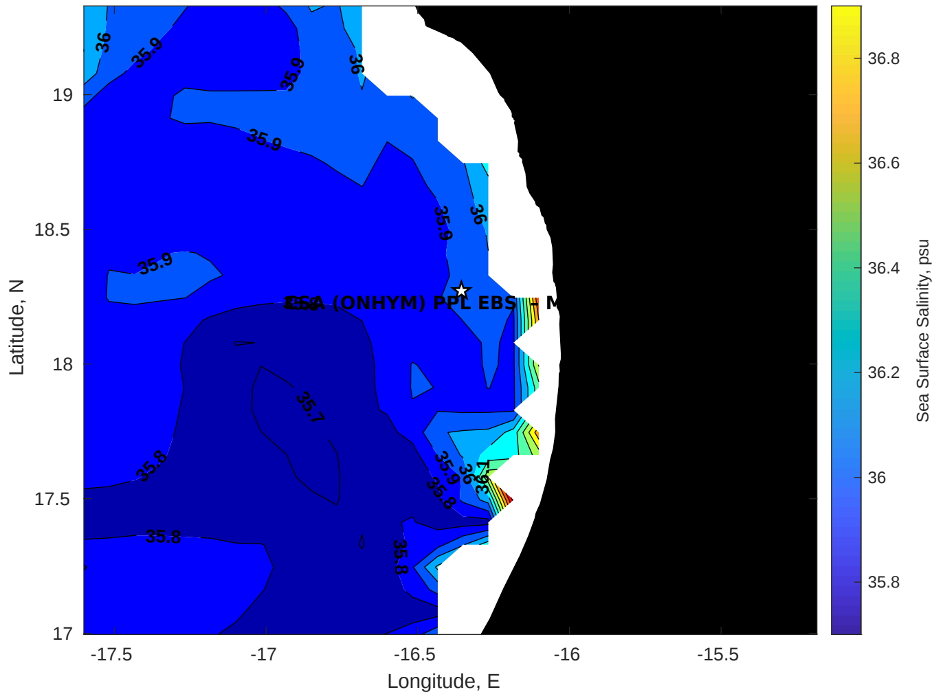
Surface Salinity for CSA (ONHYM) PPL EBS - Mauritania at 24-Apr-2025 00:00:00
