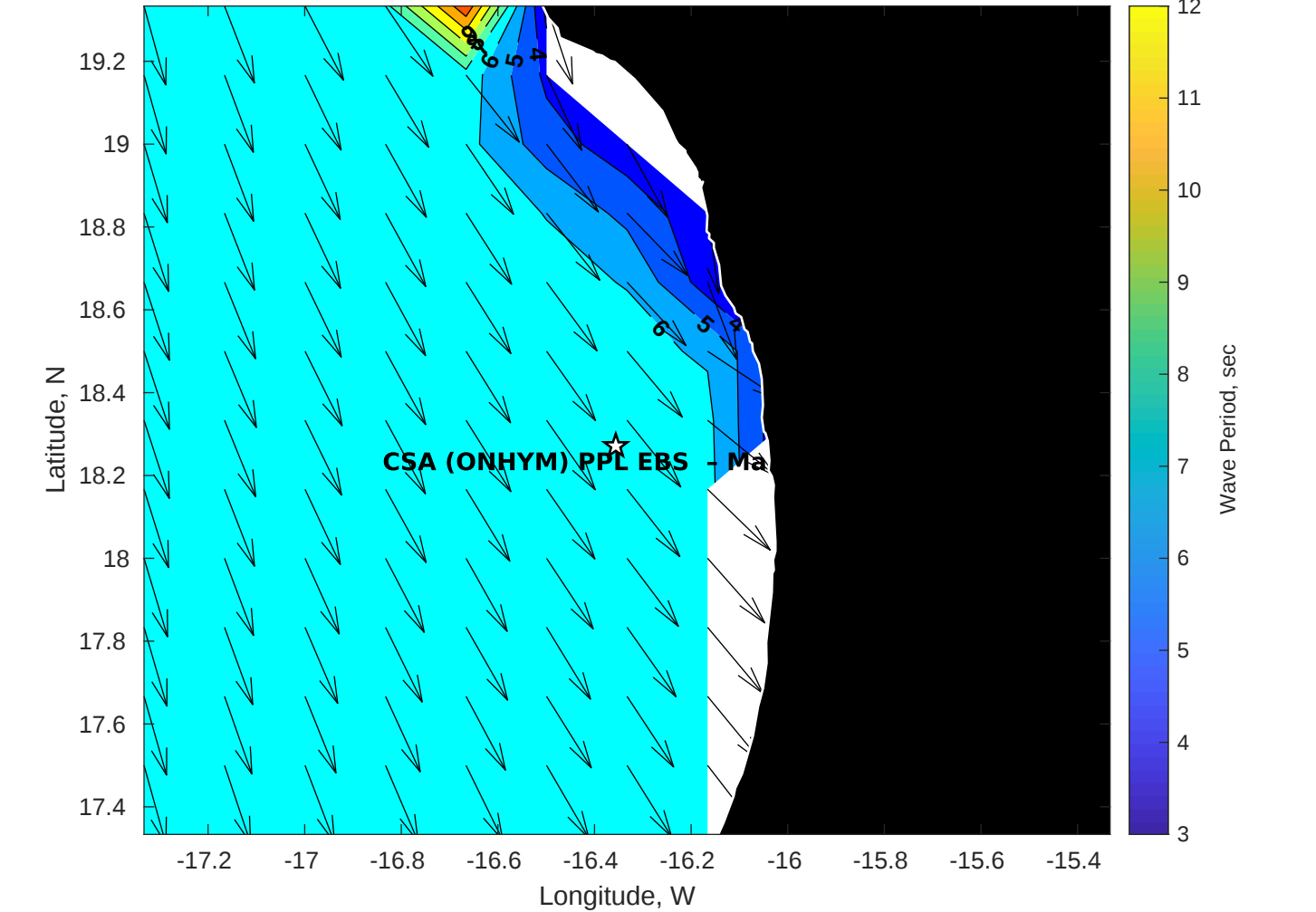
Wave Period (sec) for CSA (ONHYM) PPL EBS - Mauritania at 25-Apr-2025 09:00:00
