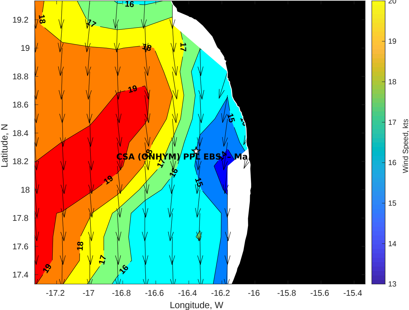
Winds (kts) for CSA (ONHYM) PPL EBS - Mauritania at 25-Apr-2025 09:00:00
