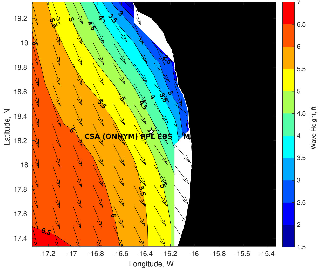
Wave Height (ft) for CSA (ONHYM) PPL EBS - Mauritania at 25-Apr-2025 09:00:00
