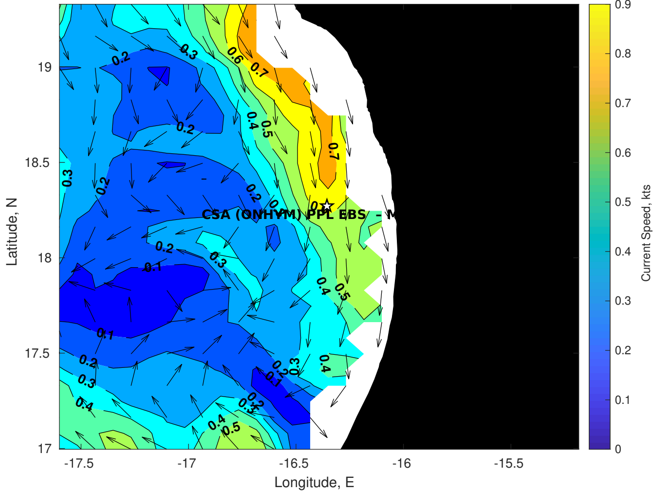
Surface Currents for CSA (ONHYM) PPL EBS - Mauritania at 24-Apr-2025 00:00:00
