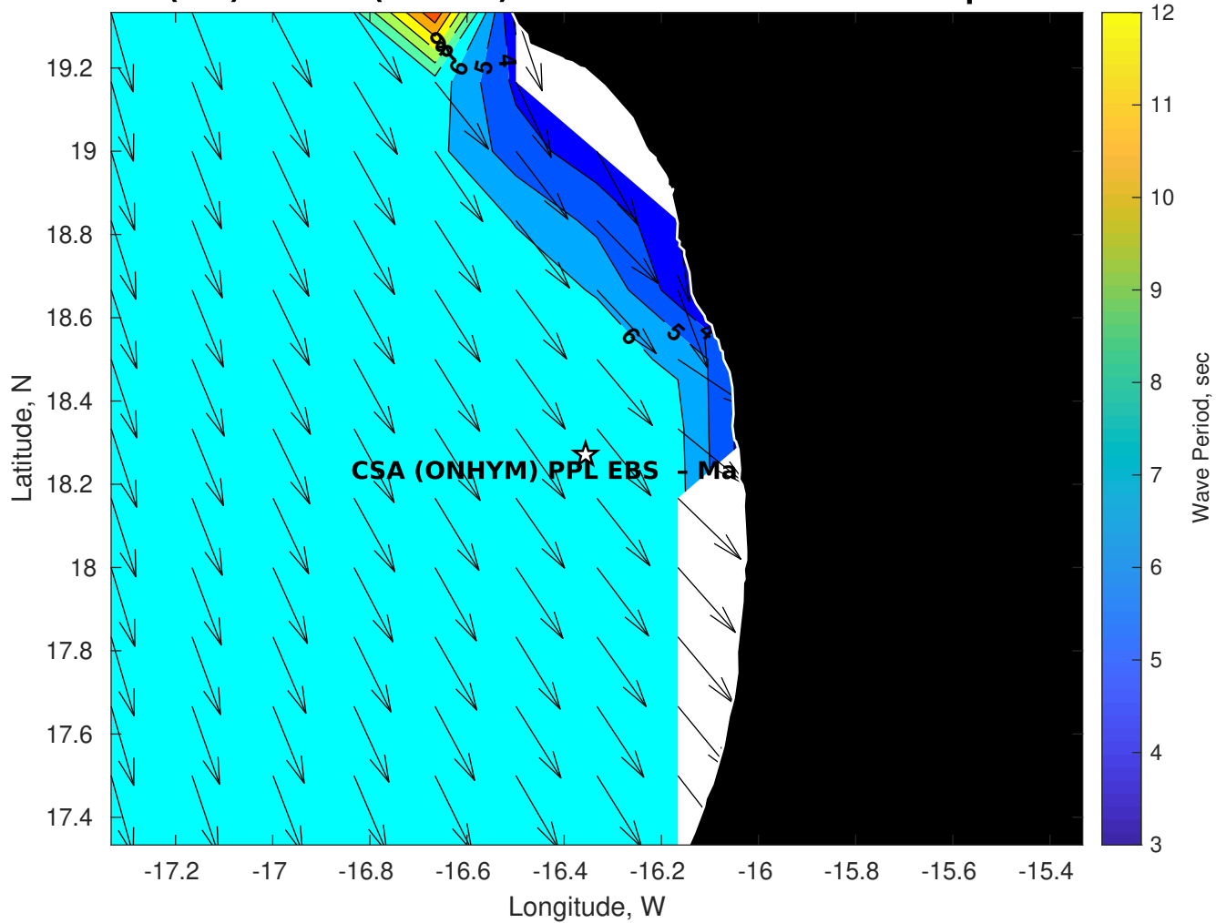
Wave Period (sec) for CSA (ONHYM) PPL EBS - Mauritania at 25-Apr-2025 09:00:00
