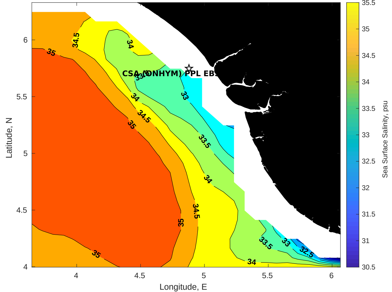
Surface Salinity for CSA (ONHYM) PPL EBS - Nigeria at 24-Apr-2025 00:00:00
