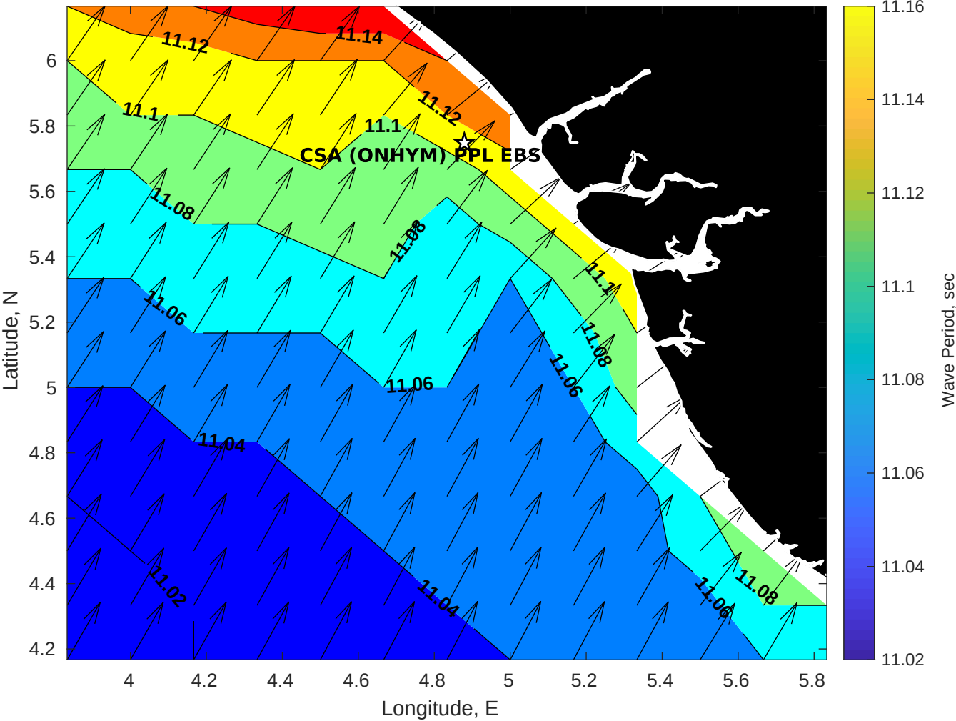
Wave Period (sec) for CSA (ONHYM) PPL EBS - Nigeria at 25-Apr-2025 09:00:00
