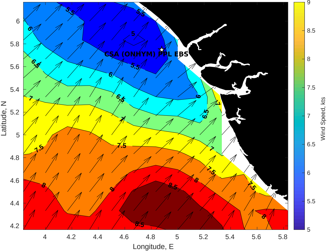
Winds (kts) for CSA (ONHYM) PPL EBS - Nigeria at 25-Apr-2025 09:00:00
