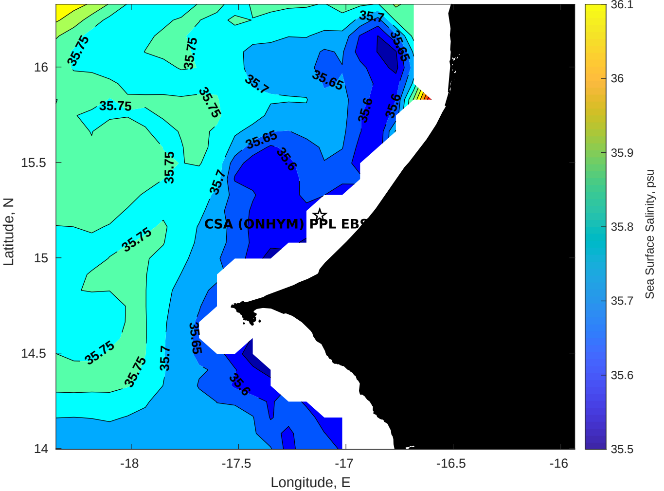
Surface Salinity for CSA (ONHYM) PPL EBS - Senegal at 24-Apr-2025 00:00:00
