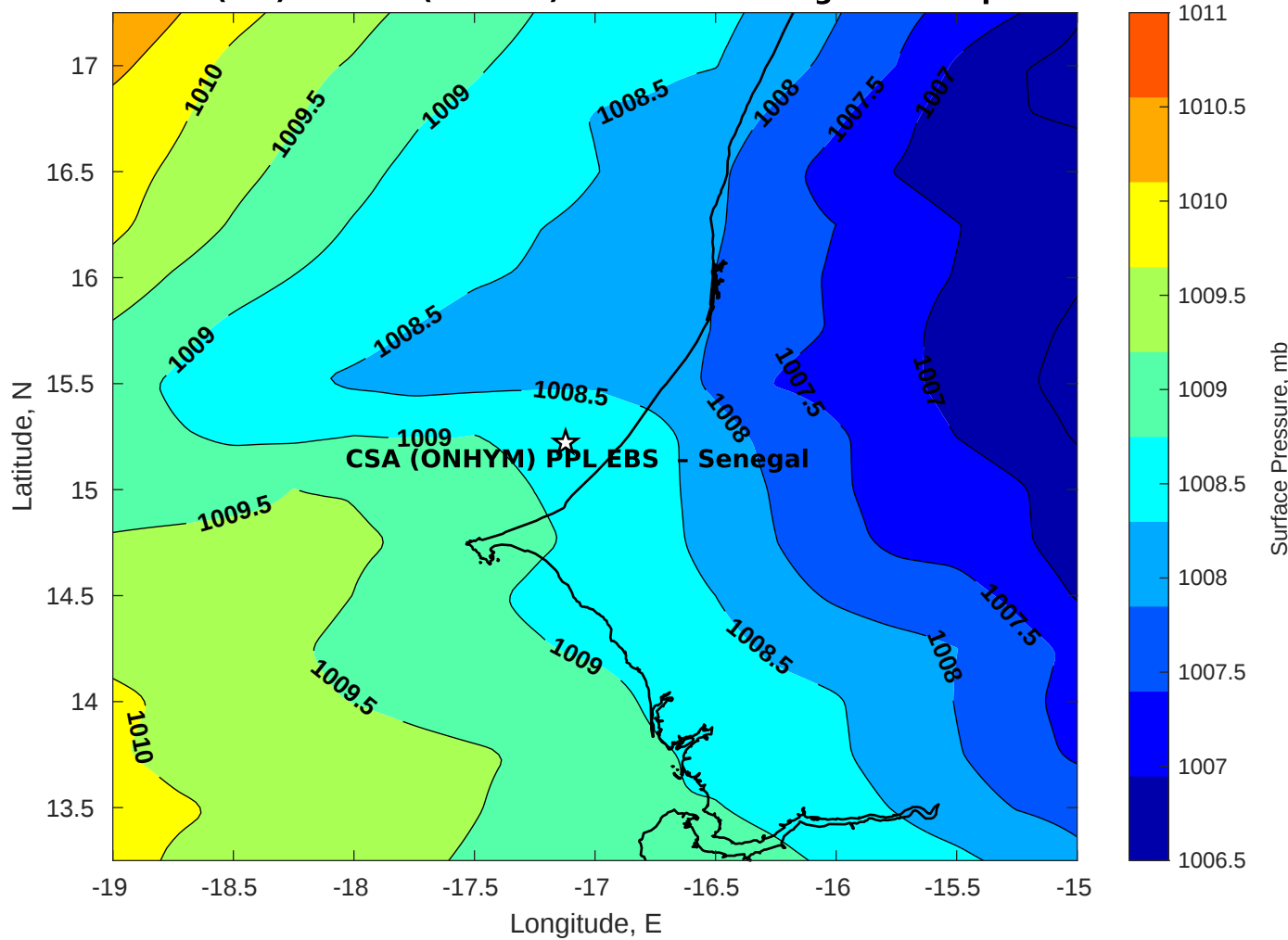
Surface Pressure (mb) for CSA (ONHYM) PPL EBS - Senegal at 26-Apr-2025 00:00:00
