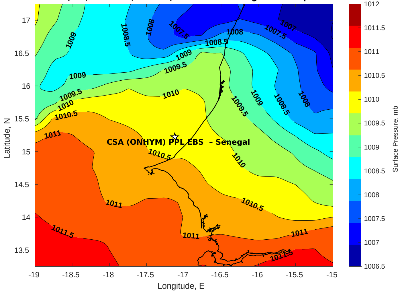
Surface Pressure (mb) for CSA (ONHYM) PPL EBS - Senegal at 27-Apr-2025 00:00:00
