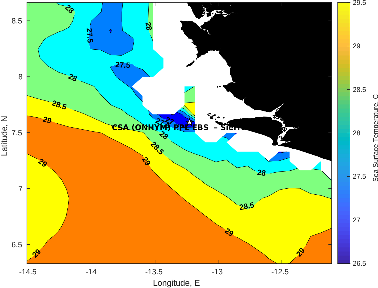
SST for CSA (ONHYM) PPL EBS - Sierra Leone at 24-Apr-2025 00:00:00
