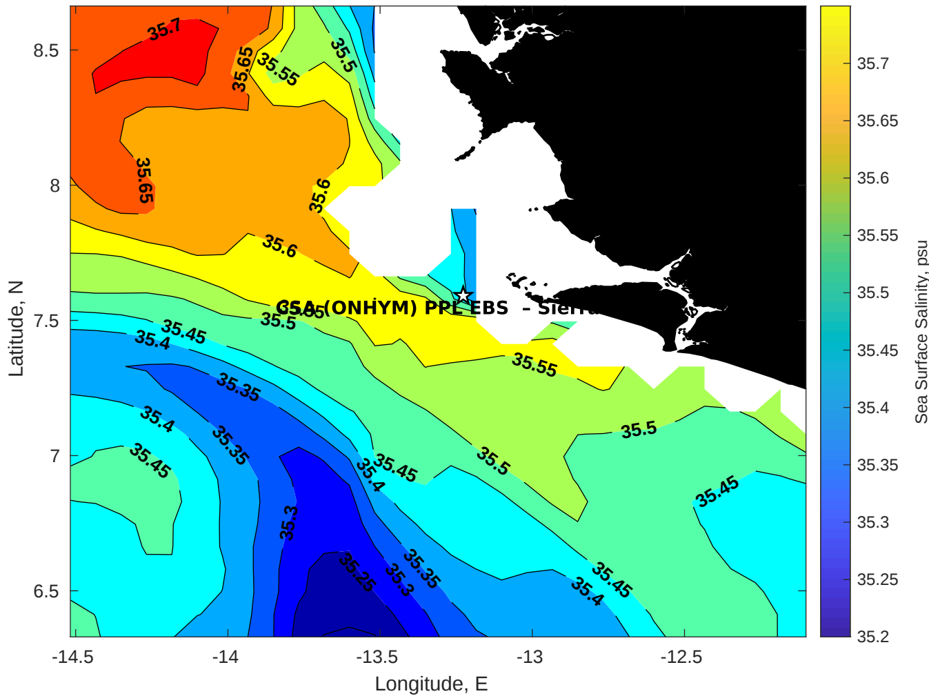
Surface Salinity for CSA (ONHYM) PPL EBS - Sierra Leone at 24-Apr-2025 00:00:00
