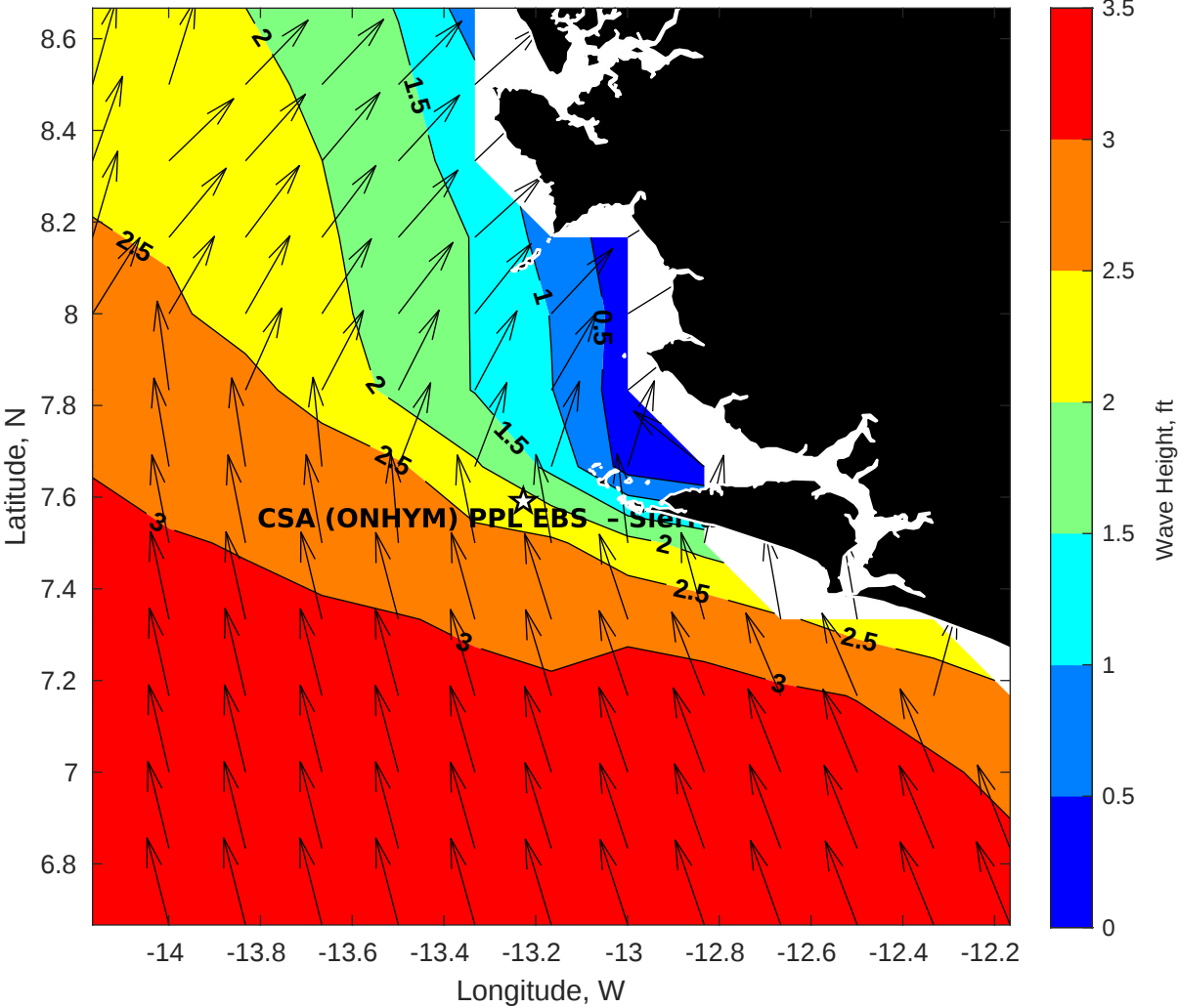
Wave Height (ft) for CSA (ONHYM) PPL EBS - Sierra Leone at 25-Apr-2025 09:00:00
