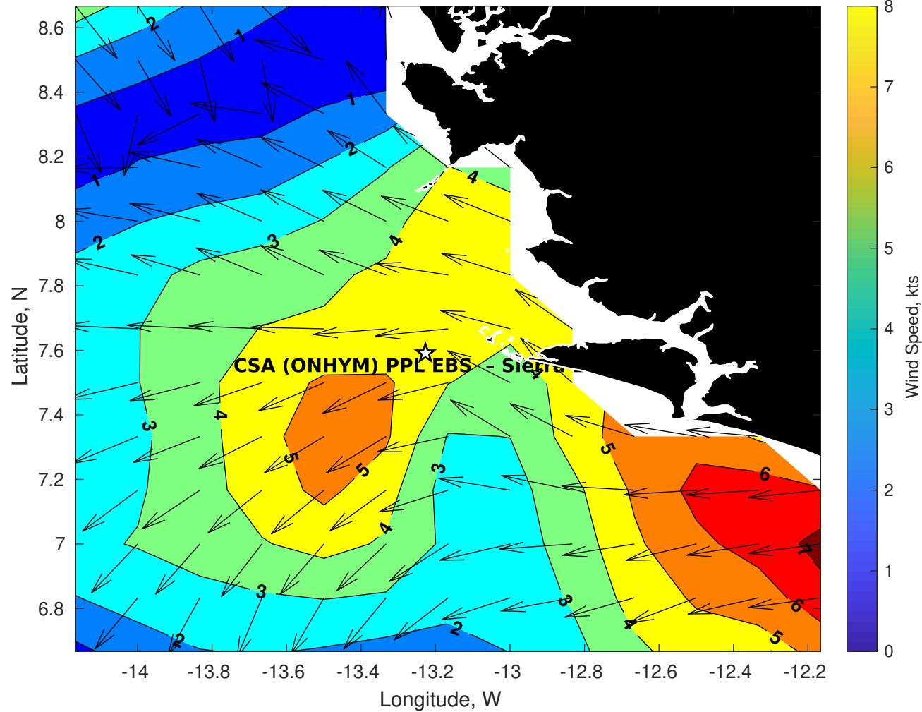
Winds (kts) for CSA (ONHYM) PPL EBS - Sierra Leone at 25-Apr-2025 09:00:00
