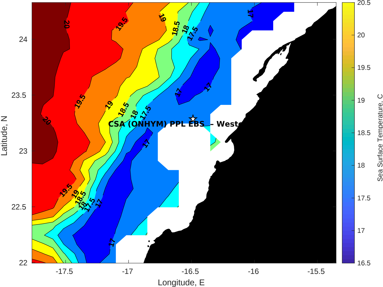
SST for CSA (ONHYM) PPL EBS - Western Sahara at 24-Apr-2025 00:00:00
