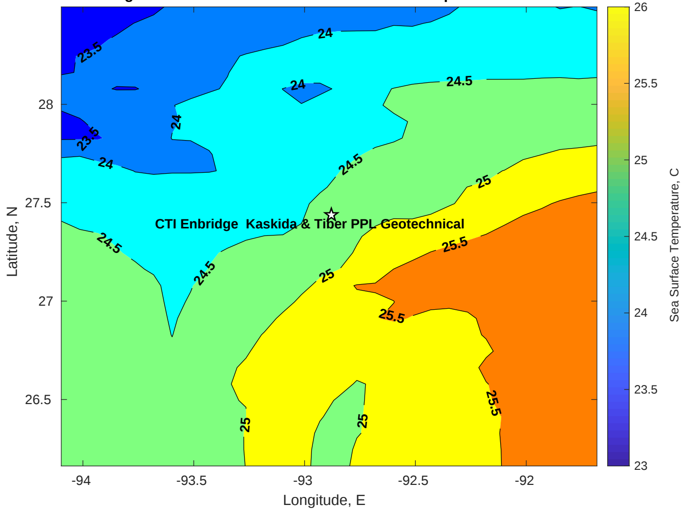
SST for CTI Enbridge Kaskida & Tiber PPL Geotechnical at 24-Apr-2025 00:00:00
